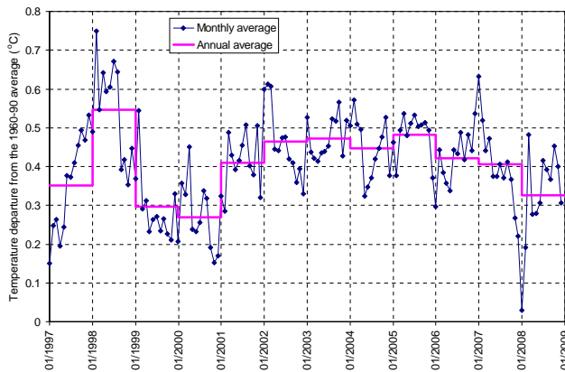
Fig. 1. Evolution of the global temperature in the last twelve years (data from CRU; combined land and marine temperatures; www.cru.uea.ac.uk/cru/data/temperature/hadcrut3gl.txt ).
