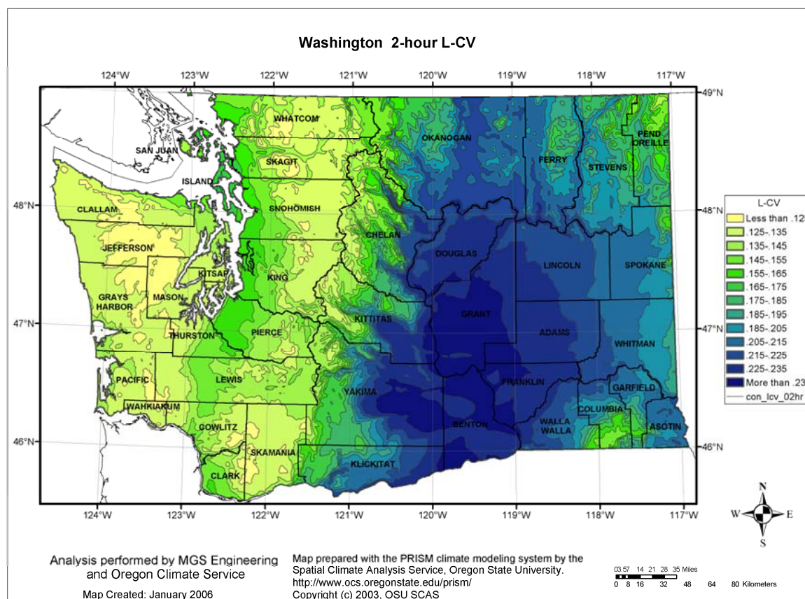
Fig. 19. Statewide variation of L-Cv annual maximum precipitation at 2-hour duration.
