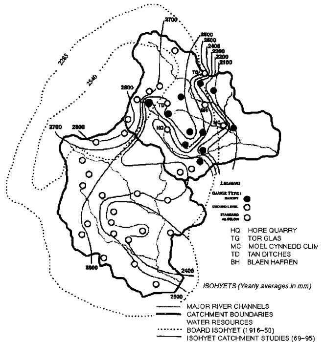
Fig. 3. The spatial distribution of precipitation in the Plynllynon catchments from the combined networks. This is compared to the regional distribution for the 1916-50 period produced by the Water Resources Board (1967), using a lower density network but incorporating gauges from outside the Plynllynon catchments.
