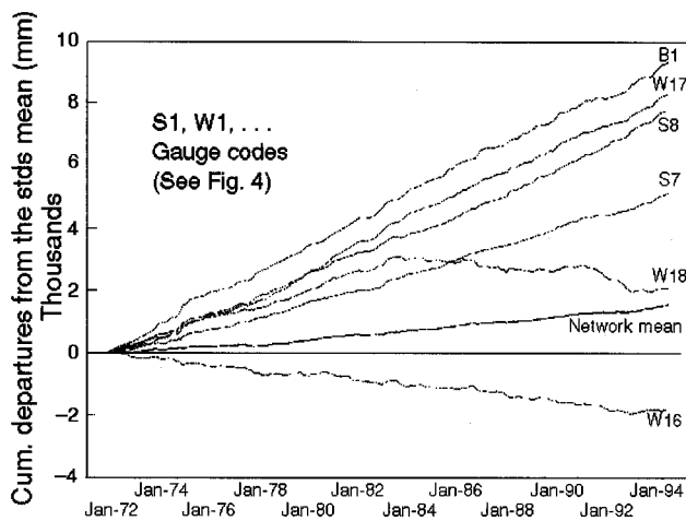
Fig. 1. Cumulative monthly precipitation departures from the standard network mean for selected high altitude gauges in the Wye catchment, illustrating the trends and the identification of problems with individual gauges (e.g. W18).
