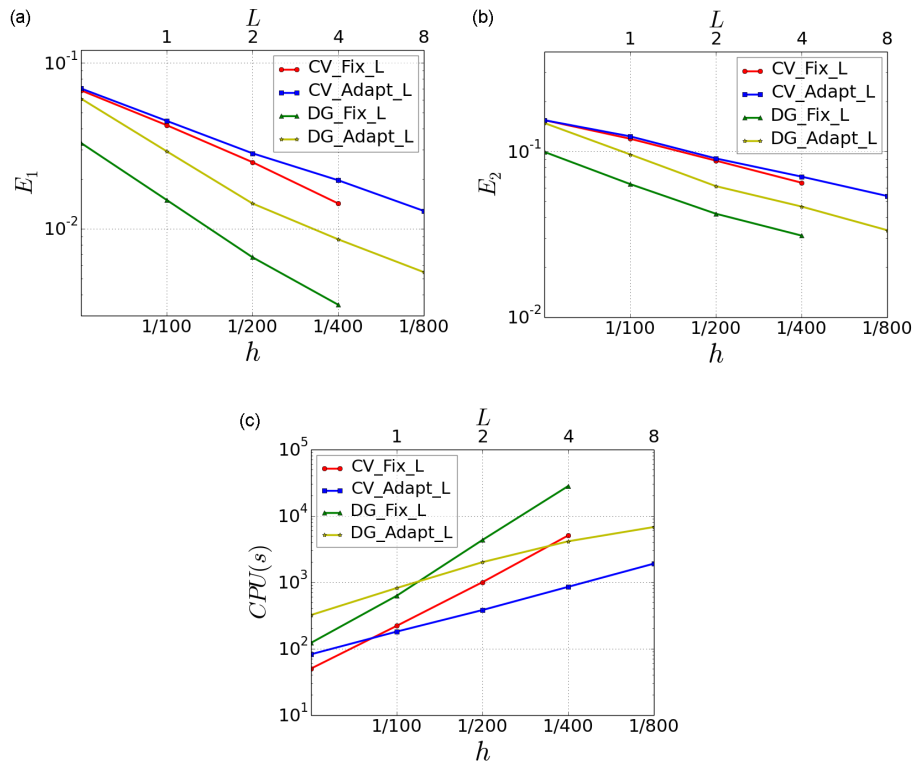
Figure 2. Case one – solid body revolution: the errors in the c field solutions and the CPU time (as a function of the mesh size h ) required for one revolution ( t = 2\pi ), where h is the mesh size for FEM_Fix_L schemes while the minimum mesh size for FEM_Adapt_L schemes.
