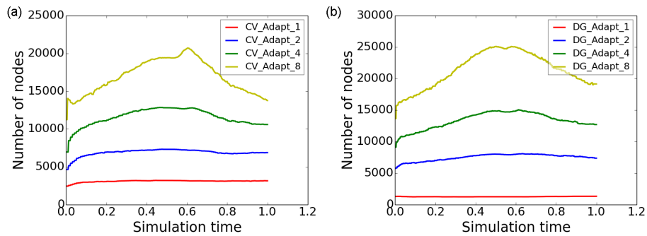
Figure 6. Case two – swirling flow: the evolution of number of nodes for (a) CV_Adapt, (b) DG_Adapt.
