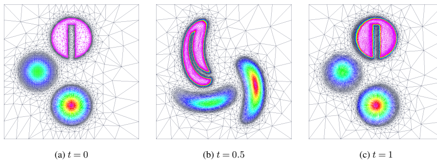
Figure 9. Case two – swirling flow: the evolution of the adaptive mesh coloured with tracer value c , where DG_Adapt_4 scheme is used.
