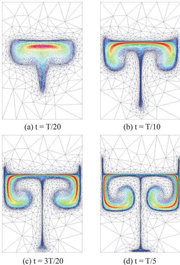
Figure 13. Case three – swirling deformation: the evolution of the adaptive mesh coloured with tracer value c , where DG_Adapt_128 scheme is used.
