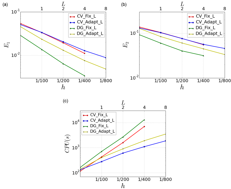
Figure 5. Case two – swirling flow: the errors in the c field solutions and the CPU time (as a function of the mesh size h ) required for one revolution, where h is the mesh size for FEM_Fix_L schemes while the minimum mesh size for FEM_Adapt_L schemes, using the same \Delta t = 0.00125 .
