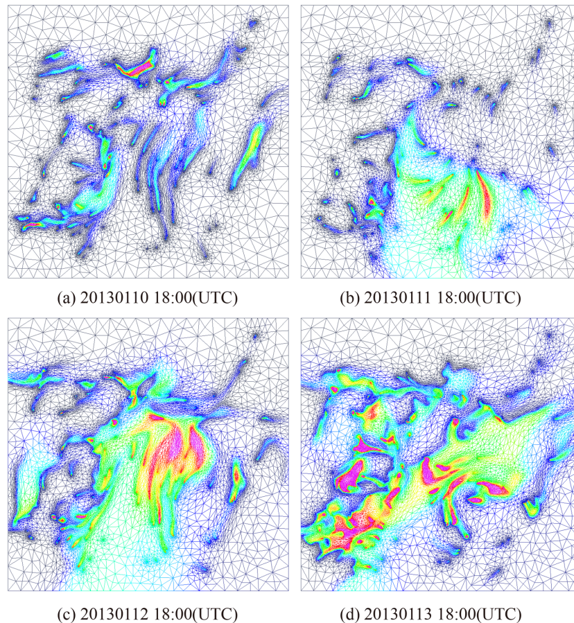
Figure 19. Case four – power plant plumes: the evolution of the adaptive mesh coloured with \text{SO}_2 concentrations ( \mu\text{g m}^{-3} ), using the CV_Adapt scheme.
