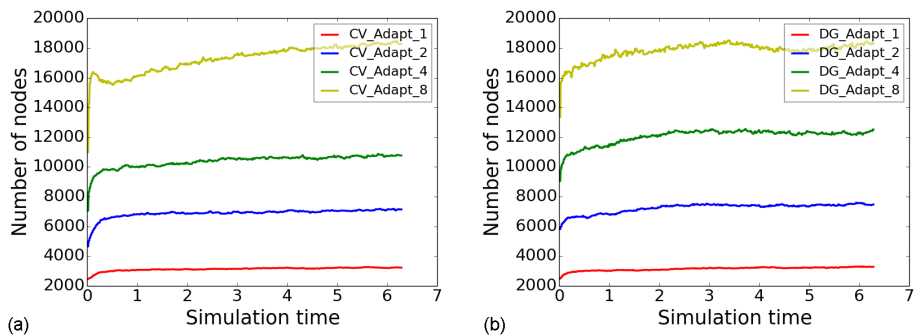
Figure 3. Case one – solid body revolution: the evolution of number of nodes for (a) CV_Adapt, (b) DG_Adapt.
