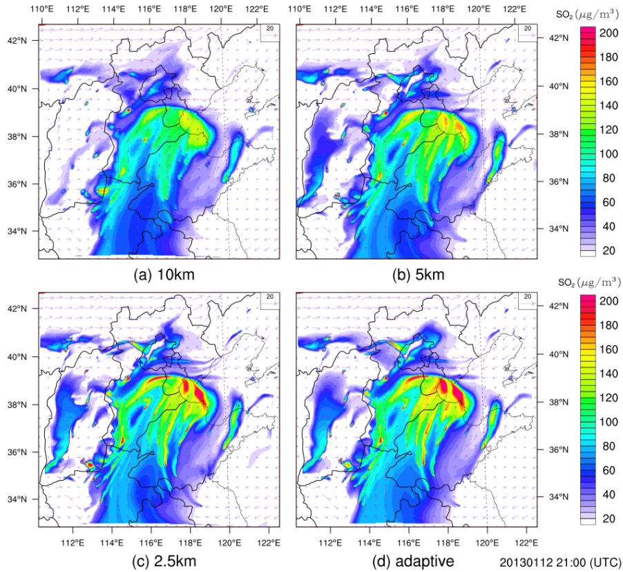
Figure 18. Case four – power plant plumes: simulated \text{SO}_2 concentrations ( \mu\text{g m}^{-3} ) at 21:00 UTC, 12 January 2013 using the CV methods on different horizontal resolution of (a) 10 km, (b) 5 km, (c) 2.5 km and on the (d) adaptive mesh.
