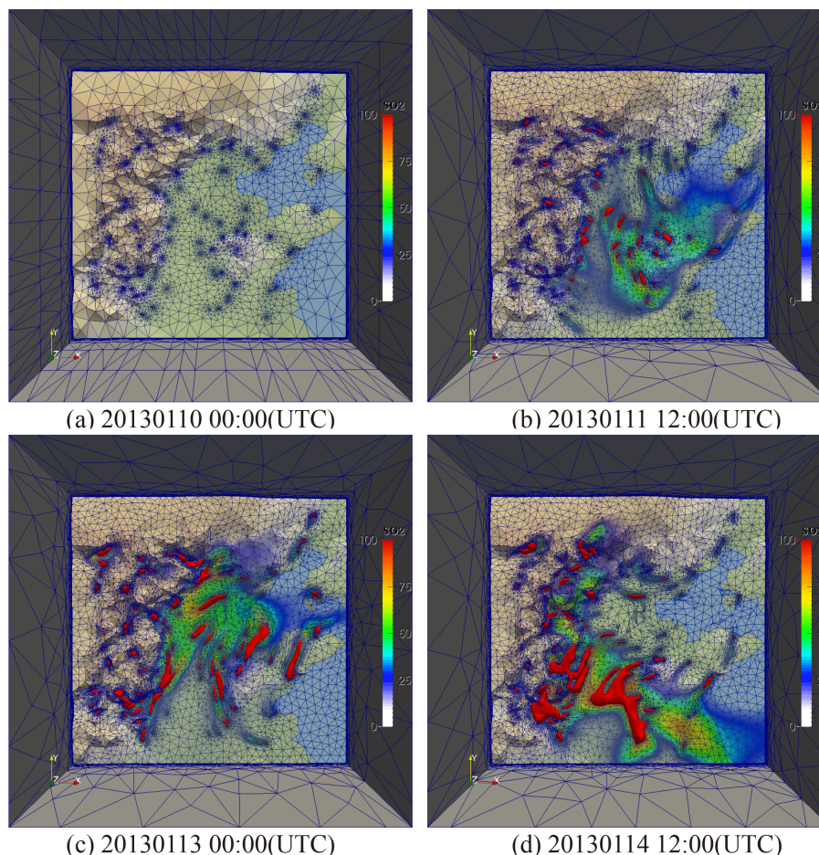
Figure 20. Case four – power plant plumes: the evolution of 3-D plumes visualization, surface \text{SO}_2 concentrations ( \mu\text{g m}^{-3} ) and the corresponding adaptive mesh.
