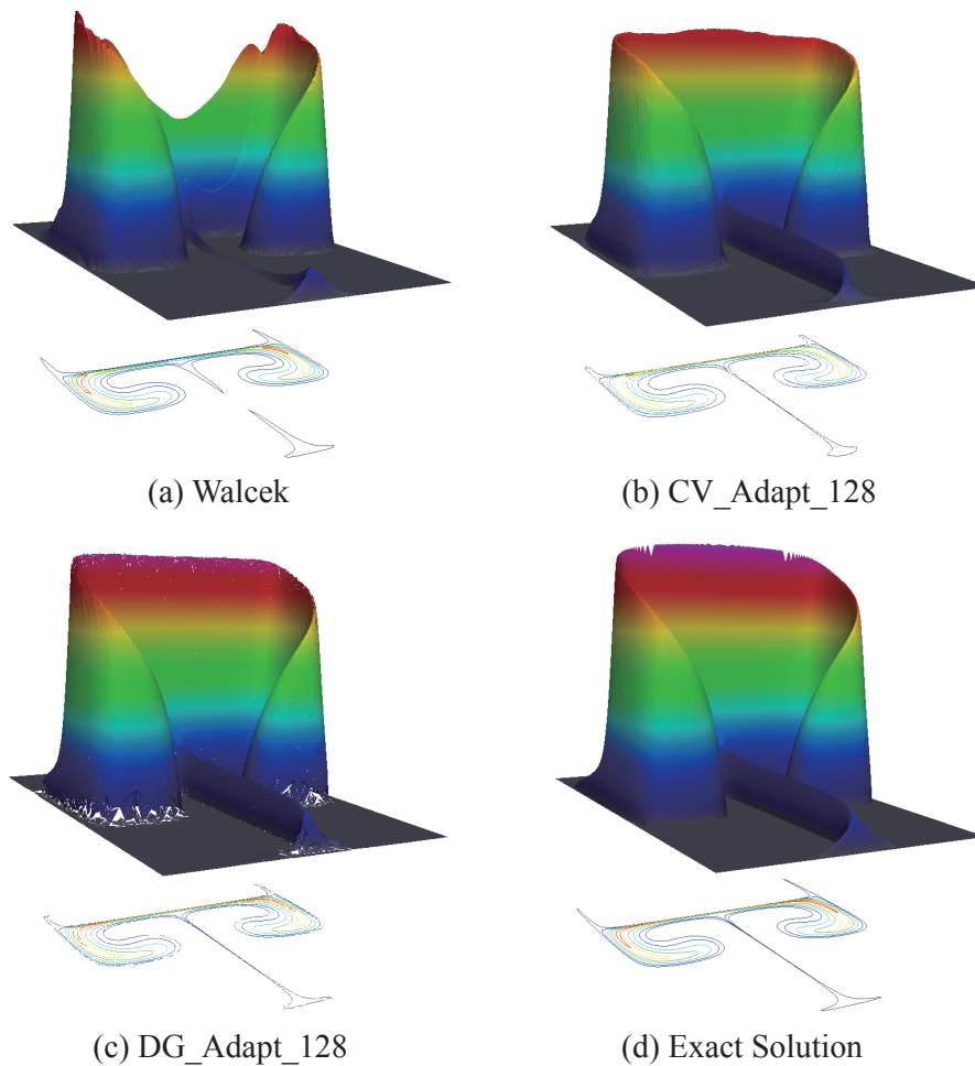
Figure 11. Case three – swirling deformation: comparison of the analytical solution with the results from different schemes using almost the same number of nodes N \approx 15\,000 , at t = 3T/20 , where T = 2.6376 .
