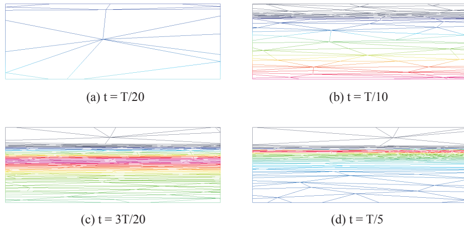
Figure 14. Case three – swirling deformation: the evolution of the adaptive mesh coloured with tracer value c , in the subdomain [0.49, 0.51] \times [0.62, 0.627] , using DG_Adapt_128 scheme.
