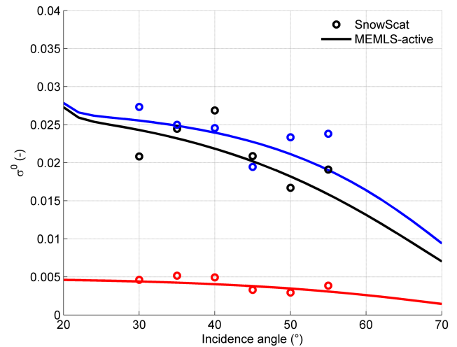
Figure 8. \sigma^0 at 10.2 GHz measured by SnowScat (circles) and modeled by MEMLS3&a with CT input (lines). Colors represent polarization, with vv – black, hh – blue and hv – red. Best fit parameters according to Fig. 7.
