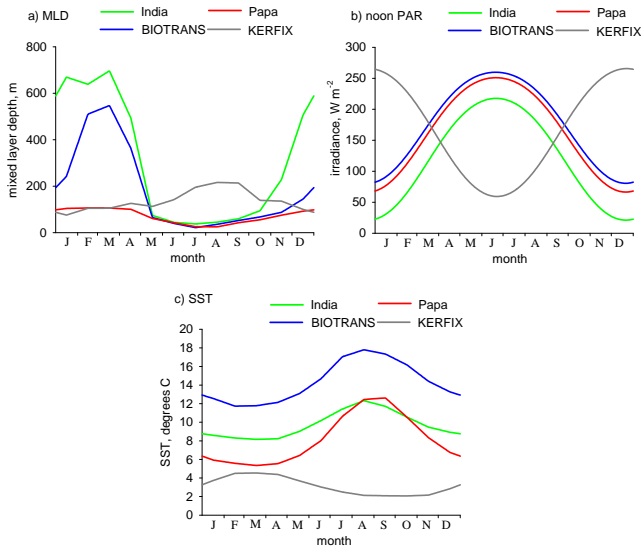
Figure 3. Model forcing for stations India ( 60^\circ N, 20^\circ W), BIOTRANS ( 47^\circ N, 20^\circ W), Papa ( 50^\circ N, 145^\circ W) and KERFIX ( 50^\circ 40' S, 68^\circ 25' E): (a) mixed layer depth (m), (b) noon irradiance ( \text{W m}^{-2} ), (c) sea surface temperature ( ^\circ C).
