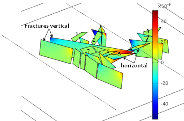
Figure 10. Distribution of the vertical fluid velocity [ \text{ms}^{-1} ] within the fracture zones at time 5900 years. The rock mass is subjected to spatially non-uniform fluid pressure and compressive stress imposed by the advancing glacier. Subhorizontal fractures are numbered 1–7.
