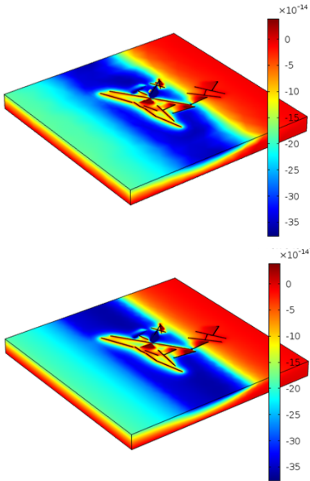
Figure 5. Vertical fluid velocity [ \text{ms}^{-1} ] in the intact part of the fractured rock for “Custom” mesh (top) and “Extra Fine” mesh (bottom). Time is 5900 years and glacier velocity is 1.27 \text{ myear}^{-1} . The velocity is obtained by solving a pure hydraulic problem.
