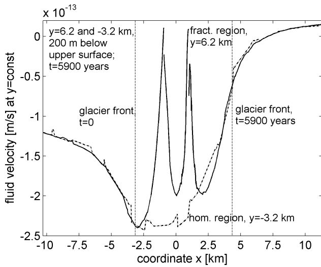
Figure 9. Vertical fluid velocity [ \text{ms}^{-1} ] in the intact part of the rock mass with fracture zones for the cross sections y = 6200 and -3200 m in the fractured and homogeneous regions, respectively, at a depth of 200 m and at time 5900 years.
