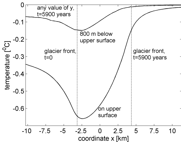
Figure 17. Temperature change [ ^{\circ}\text{C} ] in the rock mass at the upper surface and at a depth of 800 m and at time 5900 years.
