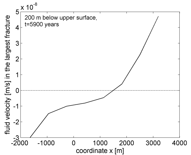
Figure 11. Variation of the vertical fluid velocity [ \text{ms}^{-1} ] in the largest fracture zone, at a depth of 200 m and at time 5900 years. Velocity is approximately uniform across the fracture's thickness.
