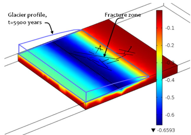
Figure 16. Temperature change distribution [ ^{\circ}\text{C} ] within the rock mass 5900 years after the start of the glacier advance.
