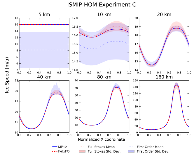
Figure 7. ISMIP-HOM test C: surface velocity component u as a function of x at y = L/4 for each L considered. The blue solid line (MP12) represents results from Perego et al. (2012) and the red dashed line (labeled FelixFO) represents results from the current solver. Note that, for the 5 km test, the MP12 and FelixFO results directly overlap the results for the full Stokes models participating in the original intercomparison.
