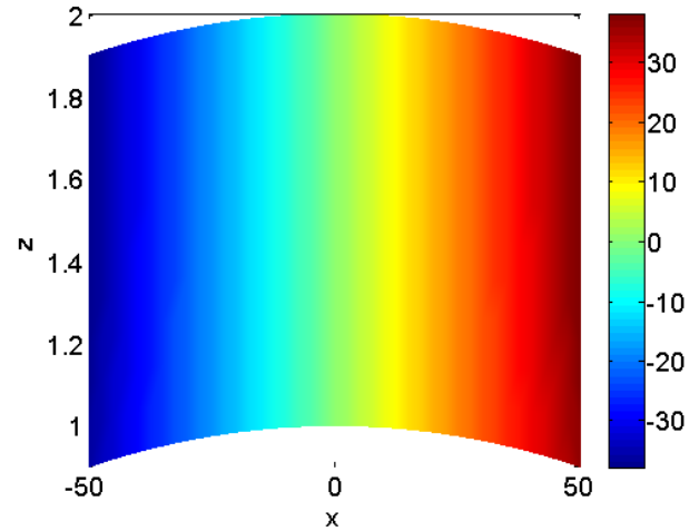
Figure 4. Contour plot of the exact solution to the x - z MMS test case.
