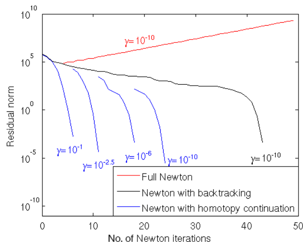
Figure 12. The robustness of Newton's method nonlinear solves with homotopy continuation.
