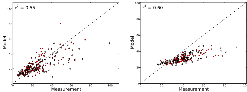
Fig. 6. Scatter plot of measured versus Polyphemus using the “rural” option, the GENEMIS temporal profile, a 15 % \text{NO}_2 fraction and stability classes based on Monin-Obukhov length (summer campaign on the left and winter campaign on the right).
