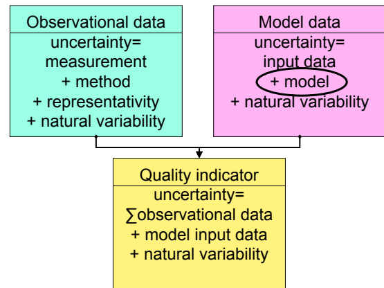
Fig. 3. Sketch, showing the components of model and observational data and the consequences for the uncertainties of the quality indicators.
