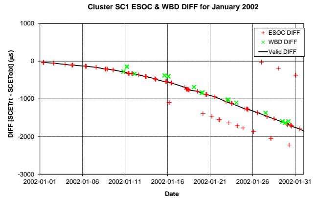
Fig. 1. Plot of the DIFF values measured by ESOC (+) and WBD (×). The solid line represents the assumed correct value used to prepare the time corrections. The “DIFF” (the difference between the ground receive time and the onboard time) is measured during every ground station contact. However some measurements are subject to errors, so a validation process must be applied.
