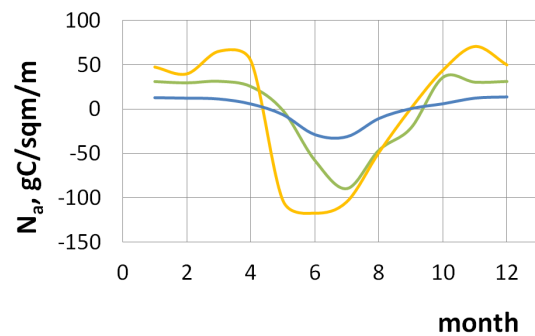
Figure 6. The seasonal cycle of the local N_{a,mod} for WUE = 2.7 \text{ gCL}^{-1} , Q_{10} = 1.4 , and \phi = 0.2 (green) as compared that for WUE = 1.8 \text{ gCL}^{-1} , Q_{10} = 2.0 , and \phi = 0 (blue) and to the detrended NEE observed at the “Hesse Forest” site of Fluxnet (orange).
