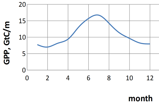
Figure 2. Seasonal cycle of the gross primary production (GPP), as calculated using Eqs. (4)–(7).
