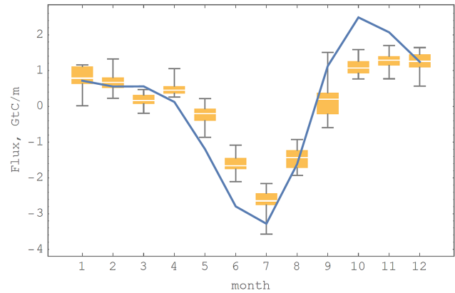
Figure 1. The seasonal cycle of the detrended net carbon exchange between the atmosphere and other pools derived from globally averaged monthly surface CO 2 concentrations in 1995–2005 (blue) as compared to the detrended TransCom 3 seasonal CO 2 flux (orange) estimated from atmospheric inversions (Gurney and Denning, 2013).
