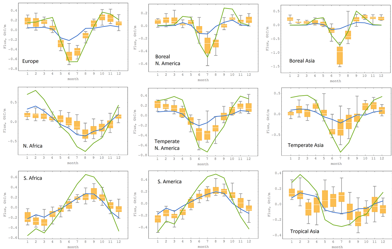
Figure 7. The seasonal cycle of the regional N_{a,mod} for WUE = 2.7 \text{ gCL}^{-1} , Q_{10} = 1.4 , and \phi = 0.2 (green) as compared to that for WUE = 1.8 \text{ gCL}^{-1} , Q_{10} = 2.0 , and \phi = 0 (blue), and to the detrended TransCom 3 seasonal CO 2 flux (orange) estimated from atmospheric inversions (Gurney and Denning, 2013).
