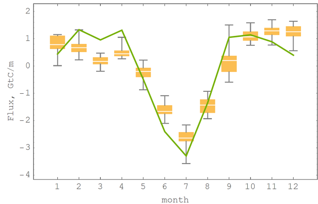
Figure 4. The seasonal cycle of N_{a,mod} (green) for WUE = 2.7 gCL -1 , Q_{10} = 1.4 , and \phi = 0.2 , as compared to the detrended TransCom 3 seasonal CO 2 flux (orange) estimated from atmospheric inversions (Gurney and Denning, 2013).
