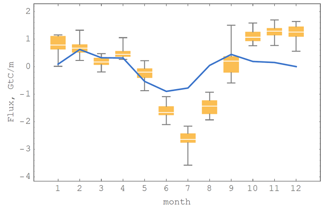
Figure 3. The seasonal cycle of N_{a,\text{mod}} (blue) for \text{WUE} = 1.8 \text{ gCL}^{-1} , Q_{10} = 2.0 , and \phi = 0 , as compared to the detrended TransCom 3 seasonal CO 2 flux (orange) estimated from atmospheric inversions (Gurney and Denning, 2013).
