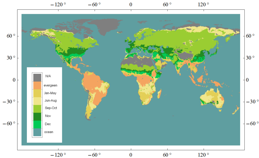
Figure 5. The month at which deciduous trees supposedly shed leaves due to the end of growing season.
