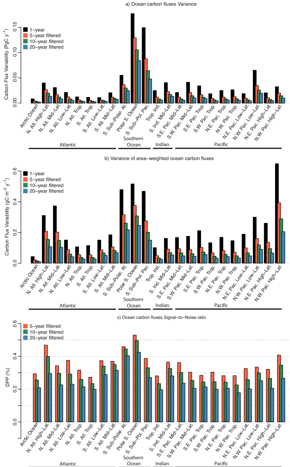
Fig. 3. Regional variability of (a) the ocean carbon uptake (in Pg C yr -1 ) and the area-weighted carbon fluxes (in g C m -2 yr -1 ) at (b) 1 yr (interannual), 5-, 10- and 20 yr time-scales. The signal-to-noise ratio (c) of these different variances is estimated by DPP metric (Eq. 2) for the various oceanic regions.
