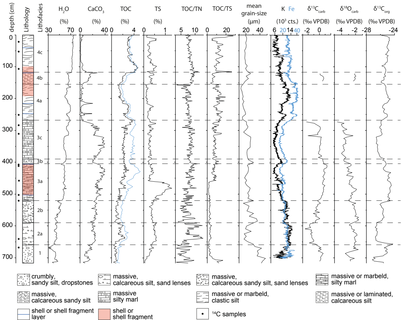
Fig. 3. Positions of 14 C samples (black dots), lithology, lithofacies, water content, calcite (CaCO 3 ), TOC (black line) and CaCO 3 adjusted TOC (blue line), TS, TOC/N, TOC/TS, mean grain-size, Potassium (K, black line) and Iron (Fe, blue line) counts, δ 13 C carb , δ 18 O carb and δ 13 C org of core Co1260.
