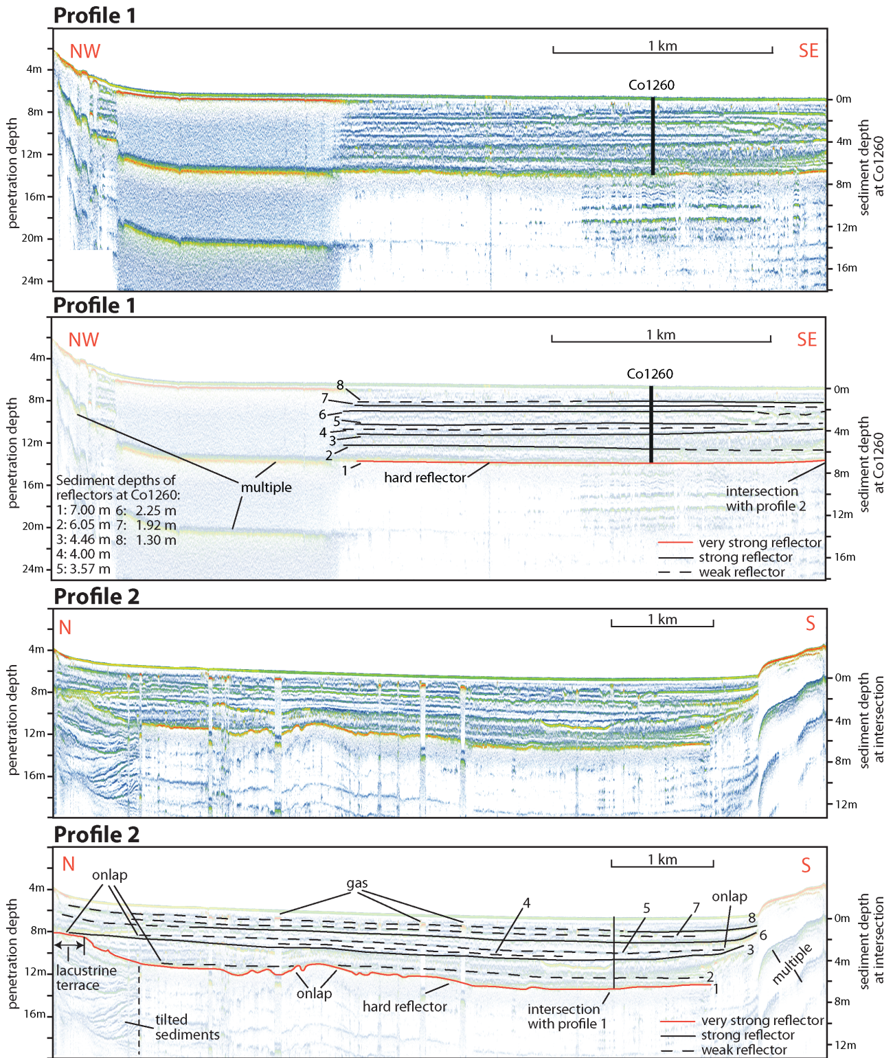
Fig. 2. Un-interpreted and interpreted hydro-acoustic profiles 1 and 2. For location see Fig. 1. The bars to the left indicates depths below lake surface, those to the right depths below sediment surface at the coring location Co1260 (profile 1) or the intersection (profile 2) between the two profiles. The length of the black bar at the coring location Co1260 corresponds to the core length.
