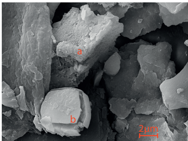
Fig. 4. SEM photos of bulk sediment from 137 cm depth in core Co1260 showing endogenic calcite ( \text{CaCO}_3 , a ) and pyrite ( \text{FeS}_2 , b ). The broken structure of the pyrite is probably due to sample pre-treatment and heating to 50^\circ\text{C} .
