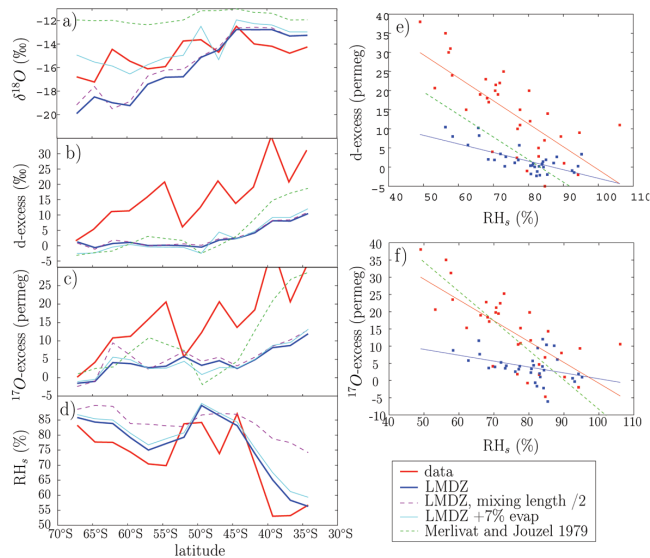
Fig. 1. \delta^{18}\text{O} (a), d-excess (b), ^{17}\text{O} -excess (c) and RH s (d) of surface water vapor measured by Uemura et al. (2008, 2010) (red) and simulated by LMDZ (blue), as a function of latitude. Results are re-gridded on the LMDZ grid and applied a smoothing Gaussian filter of 10^\circ in latitude. D-excess (e) and ^{17}\text{O} -excess (f) of surface water vapor measured by Uemura et al. (2008, 2010) and simulated by LMDZ, as a function of surface relative humidity RH s . Model outputs were collocated with the measurements. Regression coefficients for both simulated and observed values are indicated in Table 4. For comparison, the d-excess and ^{17}\text{O} -excess of surface water vapor predicted by the Merlivat and Jouzel (1979) closure approximation (Appendix A) is also shown in green. For clarity, we show only the regression line. Sensitivity tests using the LMDZ model (purple and cyan) are detailed in the text
