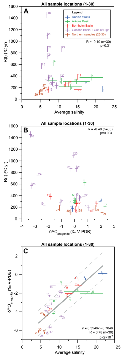
Fig. 3. (A) R(t) vs. average salinity for all samples. 1\sigma error bars. (B) R(t) vs. \delta^{13}\text{C}_{\text{aragonite}} for all samples. 1\sigma error bars. (C) \delta^{18}\text{O}_{\text{aragonite}} vs. average salinity for all samples. 1\sigma error bars. Linear regression (grey line) with 1\sigma confidence intervals (dashed line) also shown. For all figures: numbers next to data points indicate sample location numbers following Fig. 1 and Table 1.
