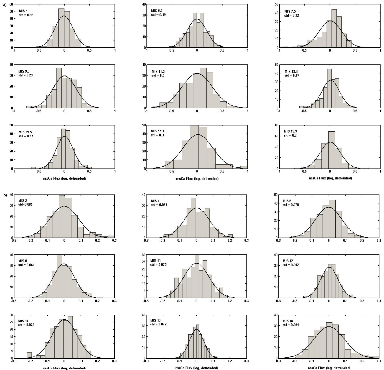
Fig. 6. Distribution during 5 kyr sections of (a) interglacials and (b) glacial periods using detrended and logarithmised 25 year mean nssCa 2+ data. The standard deviations shown are derived from the Gaussian fit.
