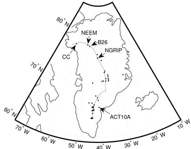
Fig. 1. The 52 ice core locations listed in Table 1. The five locations from which we have data for the most recent decade are indicated with labeled arrows.
