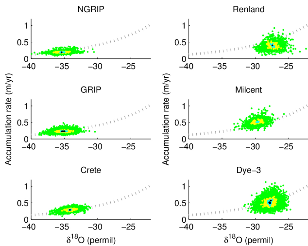
Fig. 2. Mean values of accumulation rate and \delta^{18}\text{O} for the six longest records in our data set. The averaging periods are 1 yr (green), 10 yr (yellow), 100 yr (cyan), and 1000 yr (black). The dotted grey line shows the relation from Dahl-Jensen et al. (1993) (Eq. 1). See Table 1 for the time periods covered by each data series.
