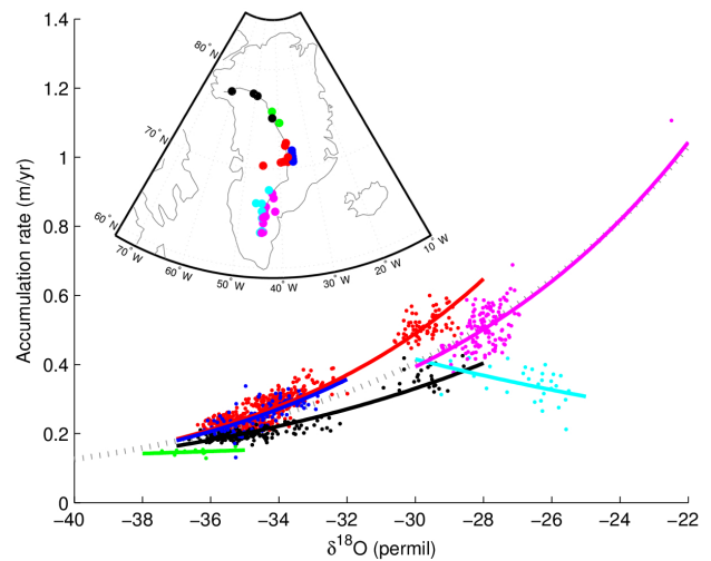
Fig. 3. 10-yr averages of ice equivalent accumulation rate and \delta^{18}\text{O} from 51 locations on the Greenland ice sheet. The records have been sorted into six groups according to location: northwest (black), northeast (green), central west (red), central east (blue), southwest (cyan), and southeast (magenta). The least squares exponential fits to the data for each of the groups in the corresponding colour and the relation from Dahl-Jensen et al. (1993) is shown for comparison (dotted grey curve). The insert shows the 51 ice core locations with colours indicating the grouping of the records. For Dye-3, data is only shown for the last 300 yr as the thickness of layers older than this are affected by upstream conditions.
