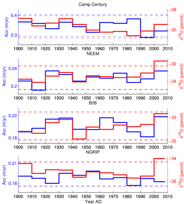
Fig. 4. Average values of accumulation rates (blue) and \delta^{18}\text{O} values (red) for each decade since 1900 AD. The blue and red dashed lines indicate the mean value \pm 2\sigma of accumulation rate and \delta^{18}\text{O} , respectively, for the whole data period for each record. The periods of data for the four records are Camp Century: 1762–2009 AD, NEEM: 1737–2009 AD, B26: 1900–2009 AD, and NGRIP: 187–2007 AD.
