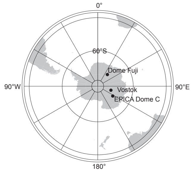
Fig. 1. Locations of the Antarctic ice cores used in this study.
