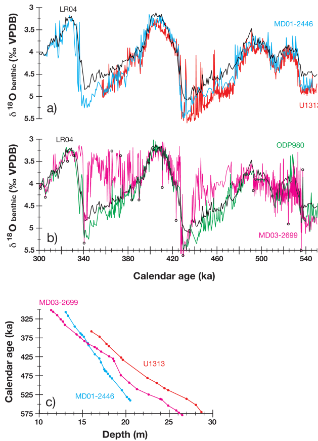
Fig. 2. (a) Benthic \delta^{18}\text{O} records of IODP Site U1313 (red) and MD01-2446 (cyan) in comparison to the LR04 stack (black) (Lisiecki and Raymo, 2005); (b) Benthic \delta^{18}\text{O} record of MD03-2699 (magenta) in comparison to ODP site 980 (green; on LR04 timescale) and the LR04 stack (black). Black circles on the MD03-2699 record mark age control points (Table 2). (c) Age-depth relationships for IODP Site U1313 and cores MD01-2446 and MD03-2699.
