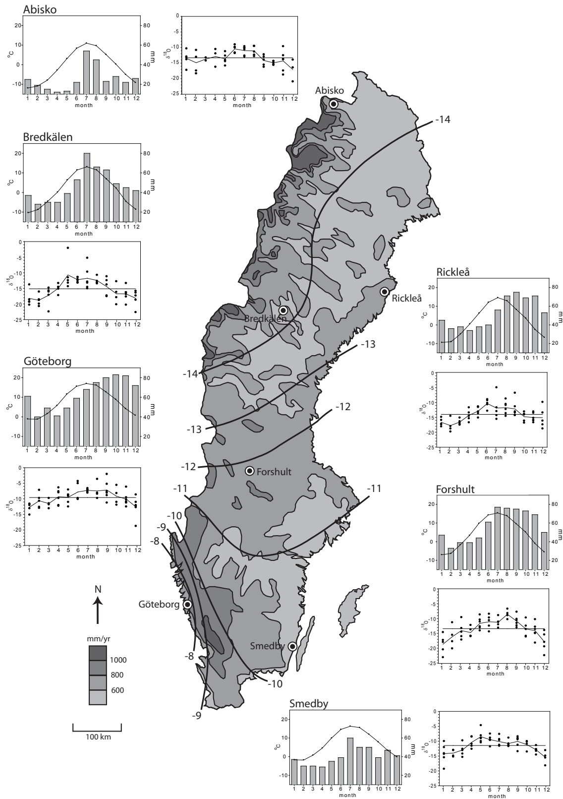
Fig. 2. Annual precipitation pattern over Sweden (Alexandersson and Andersson, 2004) and isolines of \delta^{18}\text{O} in precipitation after Burgman et al. (1987). Selected GNIP stations with monthly mean average values of \delta^{18}\text{O} in precipitation (1975–1980; IAEA/WHO) and monthly mean values of temperature and amount of precipitation from nearby meteorological stations (1961–1990; Alexandersson and Eggertsson Karlström, 2001).
