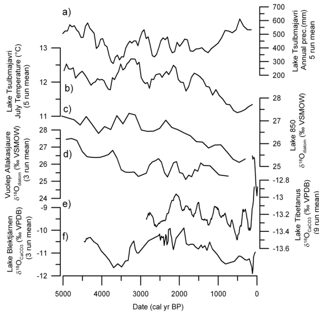
Fig. 5. Pollen inferred (a) annual precipitation and (b) July temperature from Lake Tsulbmajavri (Seppä and Birks, 2001) plotted together with \delta^{18}\text{O} records from lake sediments in Sweden: (c) Lake 850 (Shemesh et al., 2001), (d) Vuolep Allakasjaure (Rosqvist et al., 2004; Jonsson et al., 2010) and (e) Lake Tibetanus (Rosqvist et al., 2007) and (f) Lake Blektjärnen (Andersson et al., 2010). Note the different \delta^{18}\text{O} scales.
