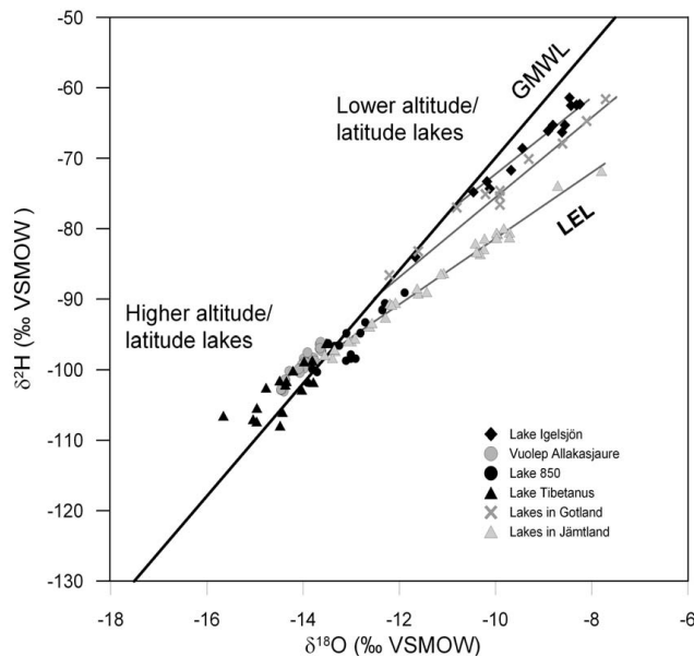
Fig. 3. \delta^{18}\text{O}_{\text{lakewater}} versus \delta^2\text{H}_{\text{lakewater}} for Vuolep Allakasjaure (Rosqvist et al., 2004; Jonsson et al., 2009), Lake 850 (Shemesh et al., 2001), Lake Tibetanus (Hammarlund et al., 2002; Rosqvist et al., 2007), Lakes in Jämtland (Andersson et al., 2010), Lakes in Gotland (Rosqvist et al., unpublished), and Lake Igelsjön (Hammarlund et al., 2003); shown in relation to the Global Meteoric Water Line (GMWL: \delta^2\text{H} = 8\delta^{18}\text{O} + 10\text{‰} ; Rozanski et al., 1993). Local Evaporation Lines (LEL) are determined from a linear regression of corresponding lake water data. Shifts along the GMWL indicate isotopic variations in precipitation input to the lake.
