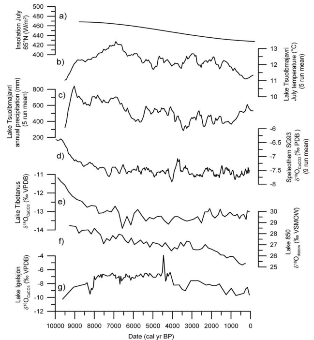
Fig. 4. (a) July insolation at 65^\circ\text{N} based on Berger and Loutre (1991) plotted together with pollen inferred (b) July temperature and (c) annual precipitation from Lake Tsuolbmajavri (Seppä and Birks, 2001). (d) Speleothem \delta^{18}\text{O} record from Norway (Lauritzen and Lundberg, 1999). Lake sediment \delta^{18}\text{O} records from (e) Lake Tibetanus (Hammarlund et al., 2002), (f) Lake 850 (Shemesh et al., 2001) and (g) Lake Igelsjön (Hammarlund et al., 2003; Jessen et al., 2005). Note the different \delta^{18}\text{O} scales.
