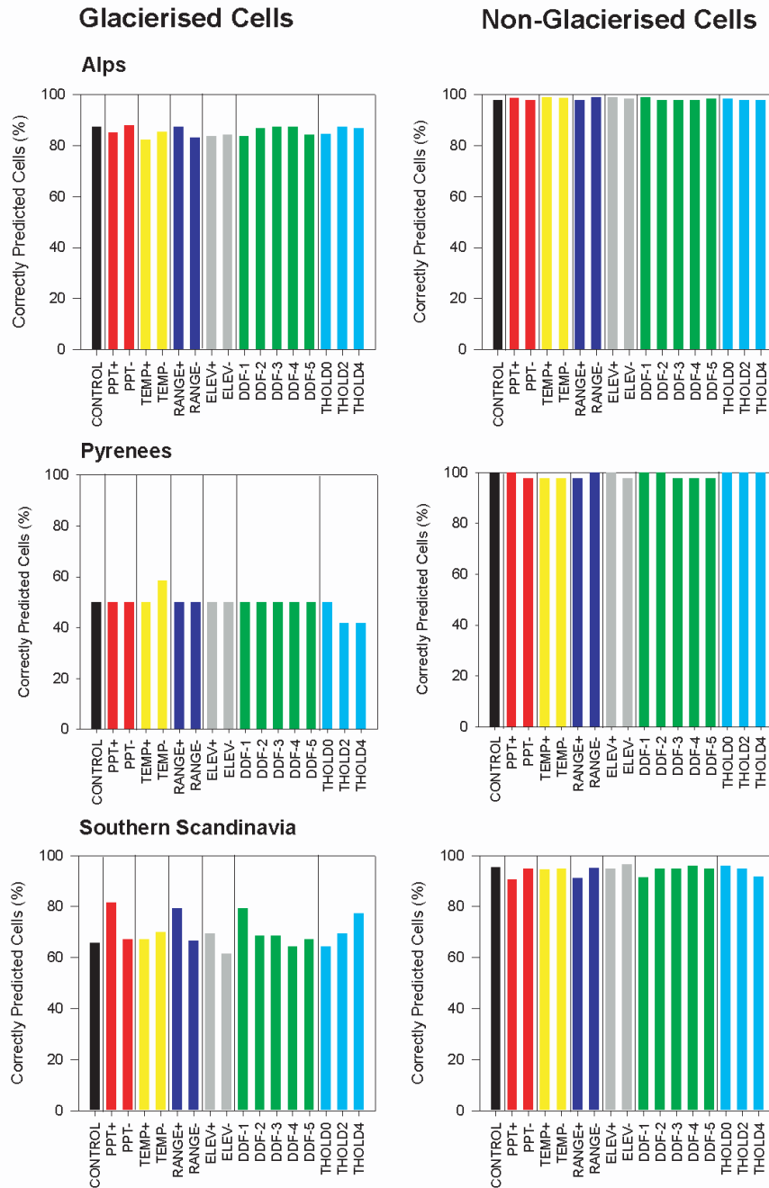
Fig. 7. Percentage of correctly predicted glacierised and non-glacierised cells across the suite of sensitivity analyses. See Table 6 for details of individual sensitivity experiments.
