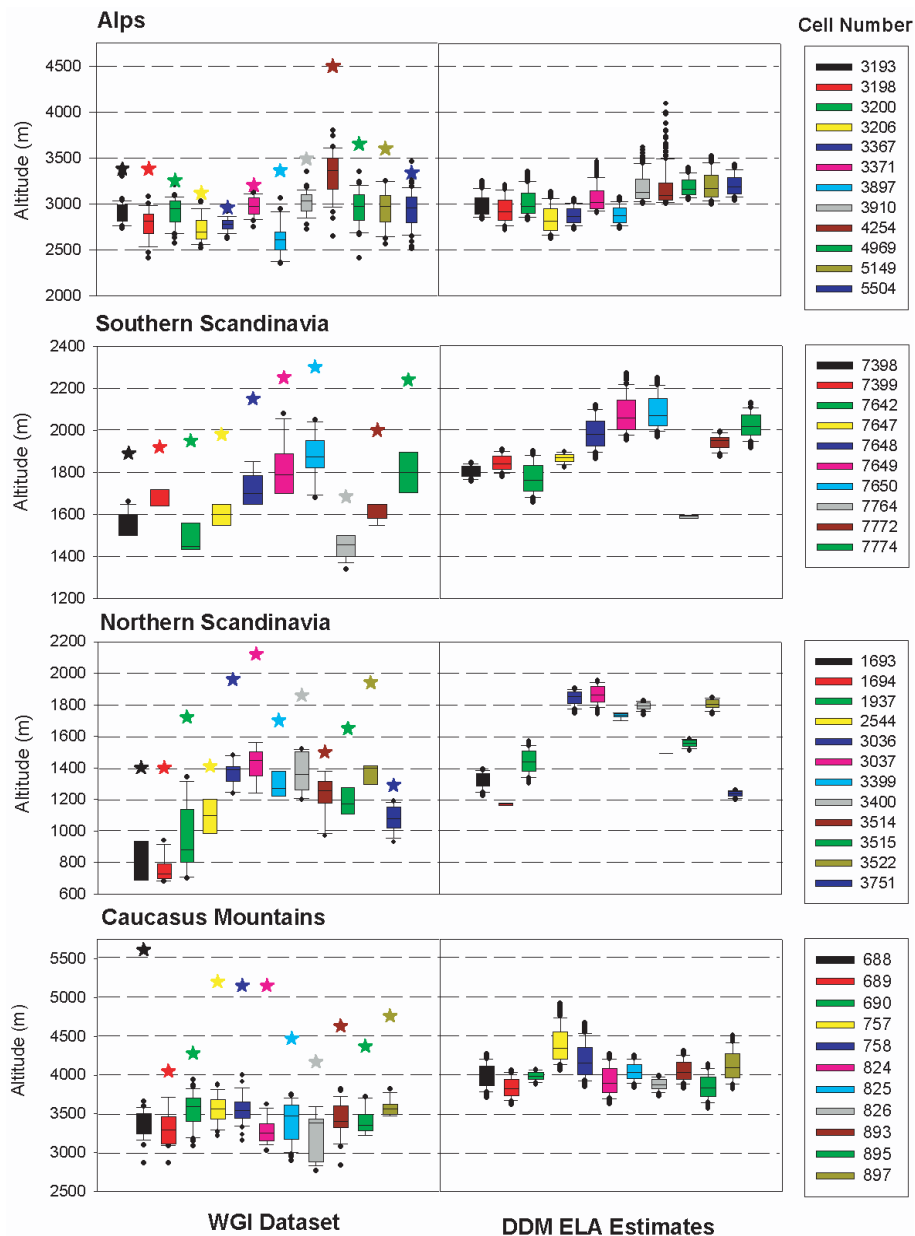
Fig. 6. WGI (National Snow and Ice Data Center, 1999) within cell altitude distributions and DDM ELA estimates. The maximum glaciated altitude in the WGI dataset is indicated by the star, the boxplot beneath the star is the altitudinal distribution of WGI snowline measurements within the cell. For identification purposes during model simulations cells in the \sim 20 km resolution model domains (see Table 3) were numbered starting from the top left hand corner of the model grid and finished at the bottom right hand corner, each row was numbered left to right. Cell numbers have been included in this diagram to help the reader compare WGI data (left hand panel) and DDM results (right hand panel) from the same cell.
