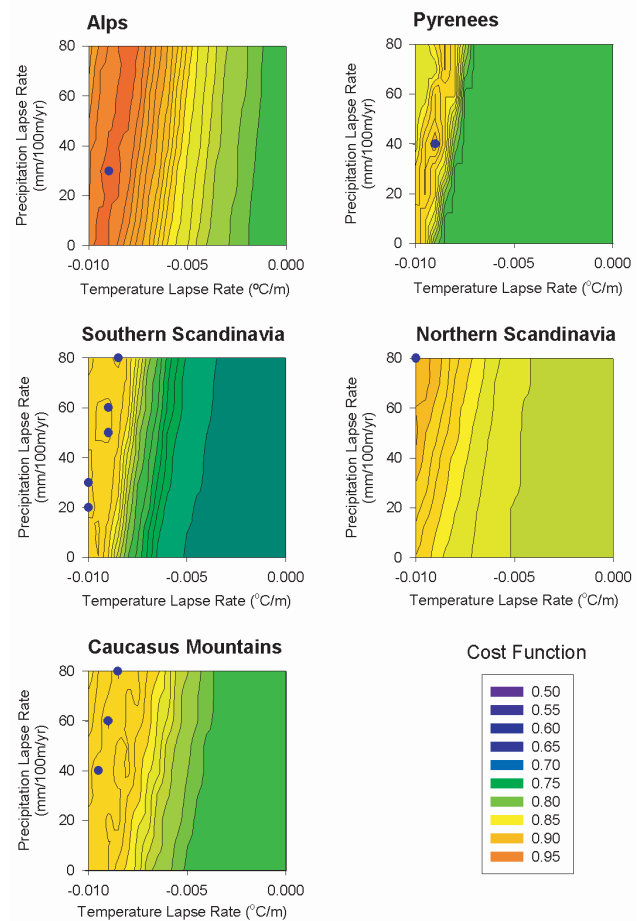
Fig. 3. Distribution of cost function results across the lapse rate domain. The blue dots are the location of the optimum temperature-precipitation lapse rate combination.
