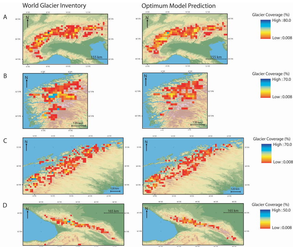
Fig. 4. Spatial distribution of glacierised cells from the WGI dataset (National Snow and Ice Data Center, 1999) and DDM simulation using the optimum lapse rate combination of the currently glacierised regions of Europe ( A =Alps, B =Southern Scandinavia, C =Northern Scandinavia, D =Caucasus Mountains) The within cell glacial coverage shown in the DDM maps are positive mass balance only. Note the maps of each region are not drawn at the same scale.
