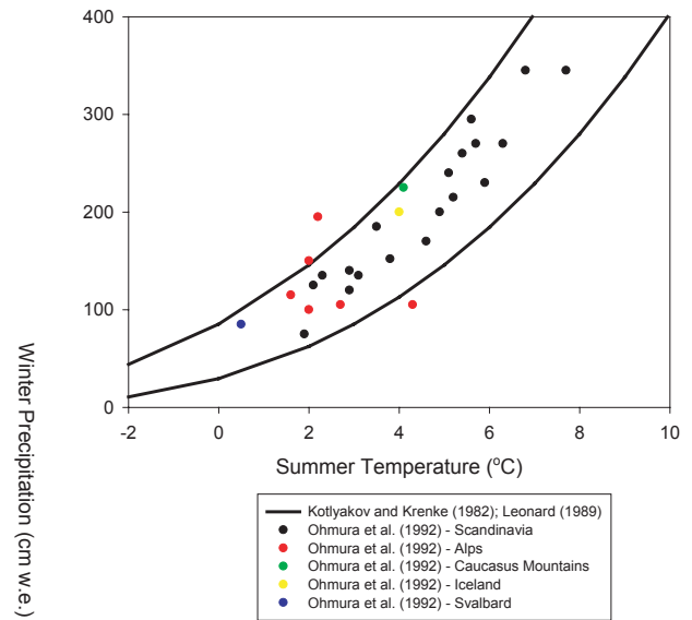
Fig. 2. ELA climates measured over mid-latitude mountain glaciers defined by Kotlyakov and Krenke (1982) and Leonard (1989). An alternative dataset of measured ELA climates (Ohmura et al., 1992) is plotted as a comparison. Apart from two Alpine ELA climates measured by Ohmura et al. (1992) the agreement between the two independently derived datasets is good and provides confidence in the use of the ELA climate “envelope” as a method for assessing DDM predictions of ELA climate.
