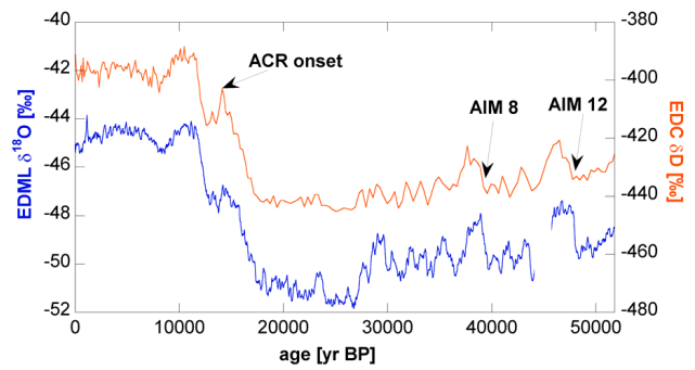
Fig. 7. EDML \delta^{18}\text{O} and EDC \delta D low resolution profiles, plotted on the EDC3 age scale after synchronisation via common volcanic signatures. The three arrows mark the three peculiar features used also in Fig. 6.
