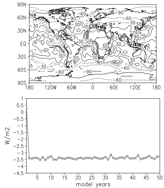
Fig. 1. The radiation balance for the control run (a) lon/lat plot averaged over the last 25 years of integration [ \text{W}/\text{m}^2 ], (b) averaged globally versus model years.
