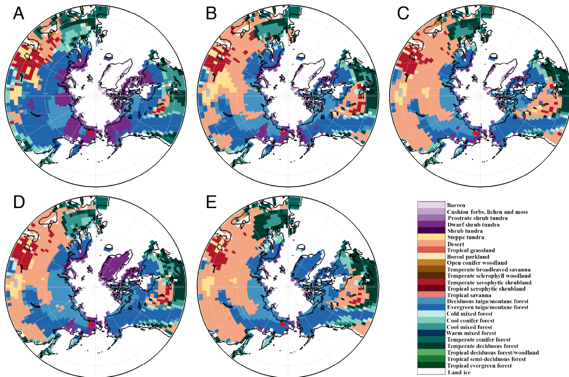
Figure 2. Distribution of interglacial vegetation simulated by the BIOME4 interactive vegetation model coupled to the GCM: (a) preindustrial vegetation corresponding to a modern orbit, (b) MIS 1 (9 ka), (c) MIS-5e vegetation, (d) MIS 11c vegetation and (e) MIS-31 (no GIS) vegetation. The location of Lake E is shown near the bottom of each figure with a red star. Note the poleward advancement of evergreen and needleleaf trees around the lake during each interglacial and the replacement of shrub tundra to taiga forest (vegetation data from Melles et al., 2012).
