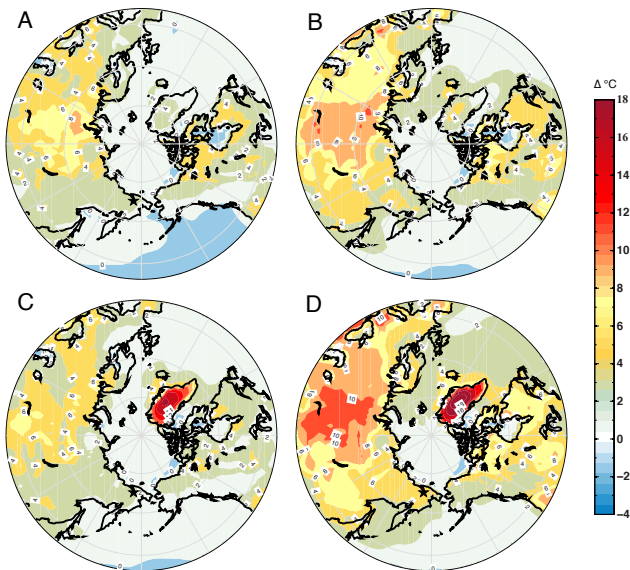
Figure 3. Simulated interglacial anomalies (2 m annual air temperature in °C) compared to preindustrial temperatures: (a) MIS 1 (9 ka orbit and GHGs), (b) MIS 5e (127 ka orbit and GHGs), (c) MIS 11c (409 ka orbit and GHGs but no Greenland Ice Sheet) and (d) MIS 31 (1072 ka orbit and GHGs but no Greenland Ice Sheet). The location of Lake E (black star) is shown near the bottom of each panel. Areas of no shading (white) roughly correspond to no change that is statistically significant at the 95 % confidence interval.
