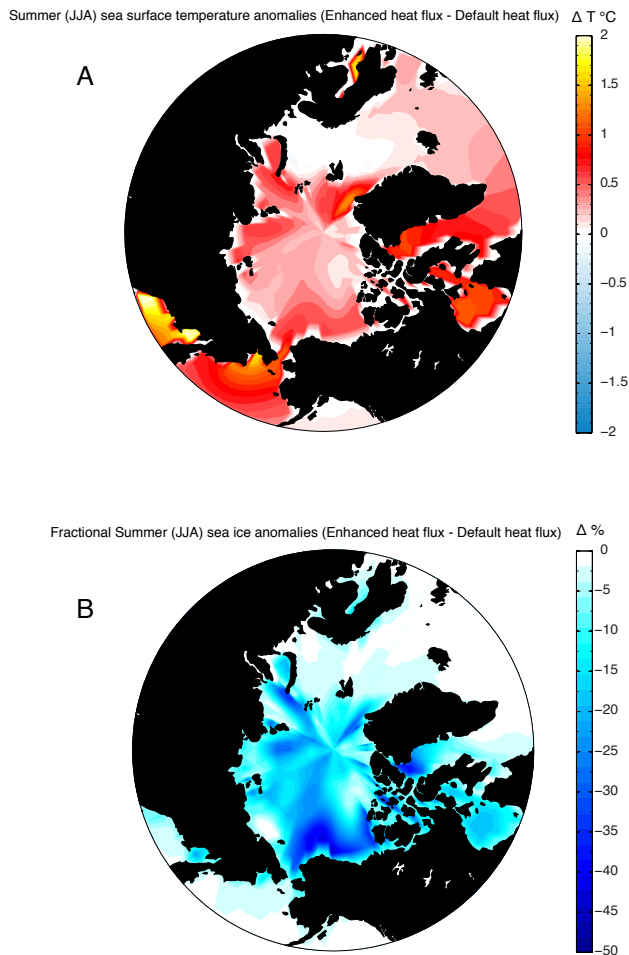
Figure 5. Model simulated (MIS11NG) summer sea surface temperature and sea ice anomalies caused by enhanced oceanic heat flux ( +8 \text{ W m}^{-2} ) at 409 ka: (a) summer (JJA) sea surface temperature change with respect to default heat flux simulation ( T \text{ } ^\circ\text{C} ) and (b) summer (JJA) sea ice fraction anomalies (%) with respect to default heat flux simulation. With +8 \text{ W m}^{-2} of subsea ice heat flux convergence, Arctic Ocean SSTs rise >0.5 \text{ } ^\circ\text{C} and sea ice fraction decreases 25–50 % in most areas.
