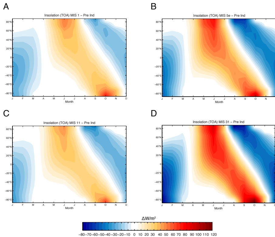
Figure 4. Monthly insolation anomalies at the top of the atmosphere for the interglacial intervals modeled here ( W m^{-2} ). (a) MIS-1 anomalies with respect to preindustrial (modern) orbit, (b) MIS-5e anomalies with respect to preindustrial orbit, (c) MIS-11c anomalies with respect to preindustrial orbit and (d) MIS-31 anomalies with respect to preindustrial orbit.
