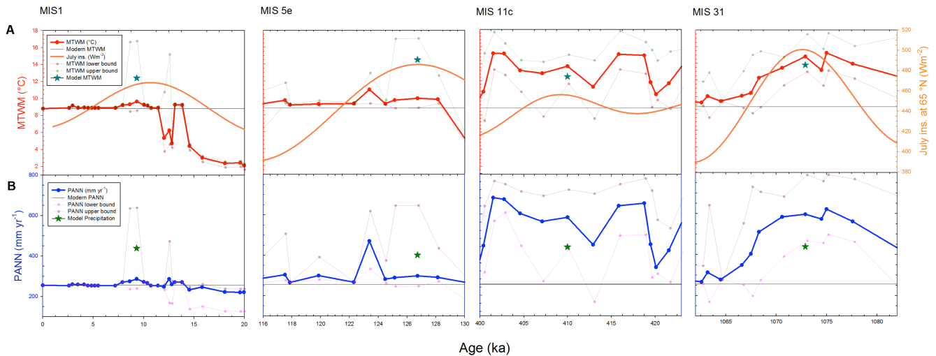
Figure 1. Reconstructed MTWM (a) and PANN (b) from Melles et al. (2012). Transparent data above and below the bold lines are upper and lower limits of each data point calculated from a best modern analogue technique (MAT) function. The dark cyan (in a) and dark green (in b) stars denote results from the GCM simulations with respect to MTWM and PANN.
