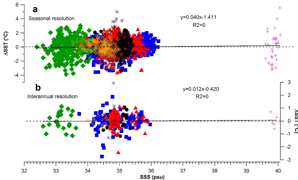
Figure 2. \Delta\text{SST} ( =\text{SST}_{\text{Sr/Ca}}-\text{SST}_{\text{I}} ) plotted against salinity (SODA SSS product v2.2.4, Carton and Giese 2008) at seasonal (a) and interannual (annually averaged time series) (b) resolution for all coral data. Green diamonds: eastern tropical Pacific; blue squares: western tropical and subtropical Pacific; brown stars: western subtropical North Pacific Ocean; red triangles: central tropical Pacific; black circles: Indian Ocean; pink crosses: Red Sea; yellow diamonds: Indonesian region.
