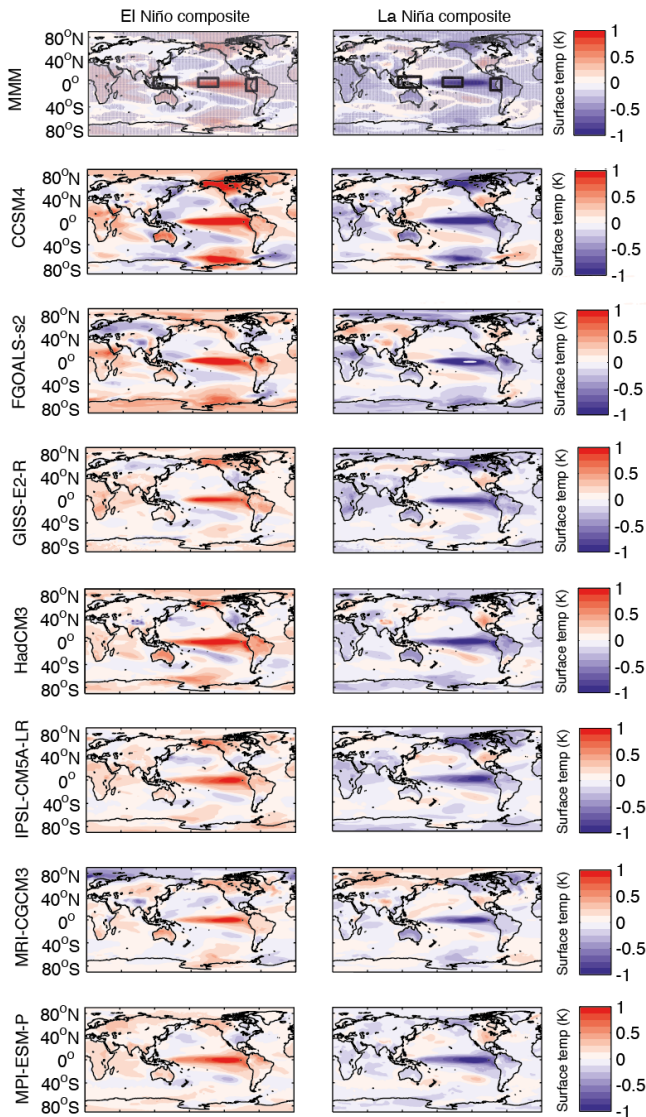
Figure 2. As for Fig. 1, but showing composites from Last Millennium experiment.
