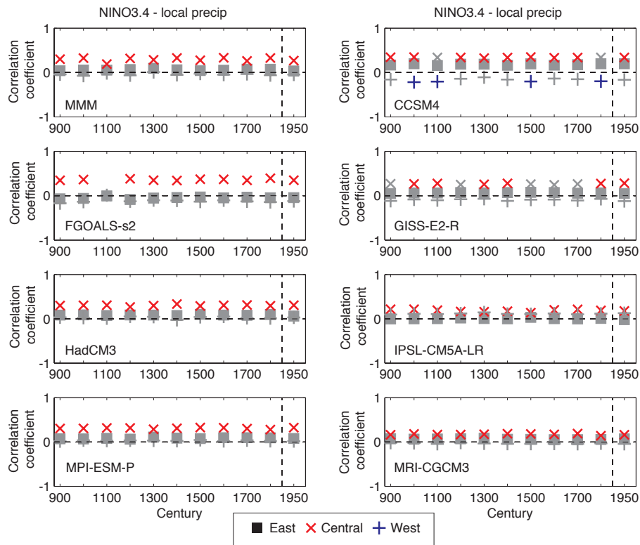
Figure 8. As for Fig. 7 but showing correlation coefficients ( R ) of NINO3.4 and local precipitation.
