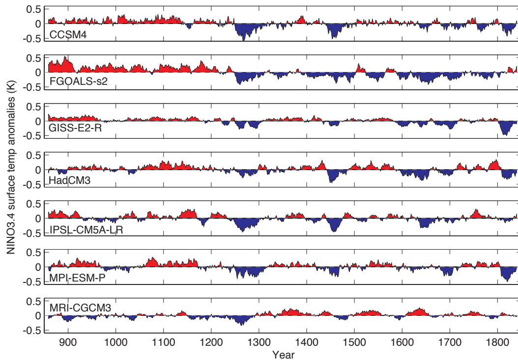
Figure 5. Running annual-mean surface temperature anomalies (K) over the NINO3.4 region ( 5^{\circ} N– 5^{\circ} S, 170^{\circ} – 120^{\circ} W) for Last Millennium simulation for each model. Red/blue shading highlights departures from each model’s long-term mean. Running means were calculated using a 240-month triangle smoother.
