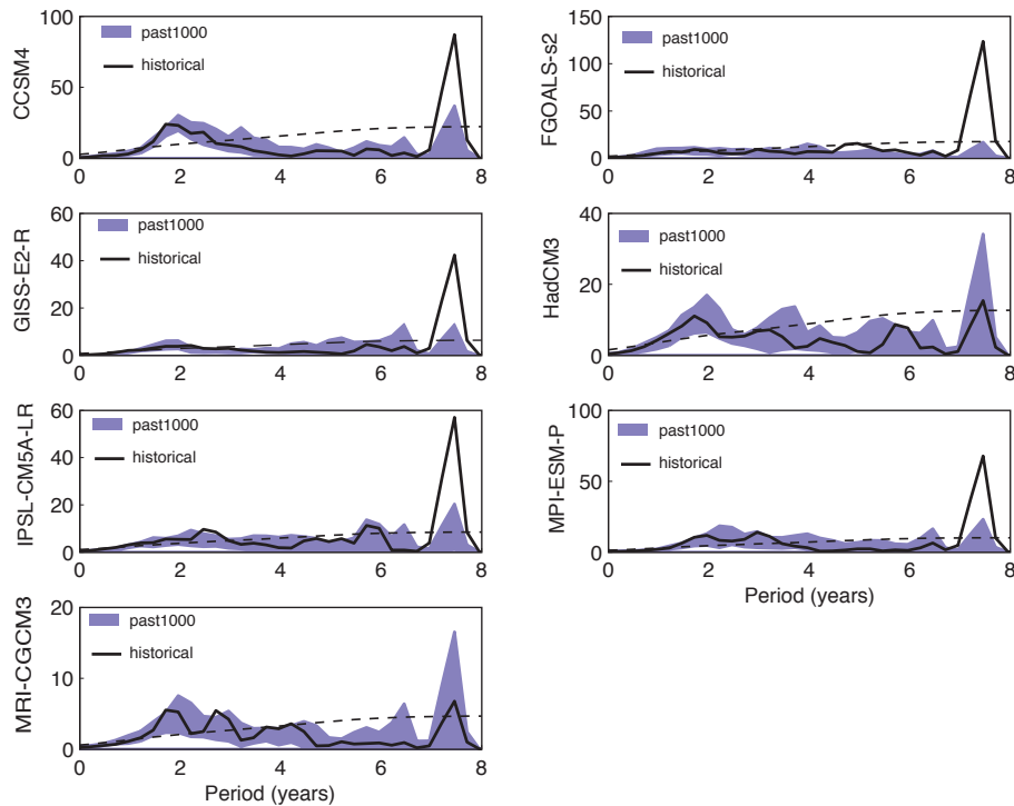
Figure 4. Global mean NINO3.4 power spectrum ( K^2 /unit frequency, black) of Last Millennium simulations, relative to the red-noise (AR(1)) benchmark (dashed), for the multi-model mean (MMM) and each model analysed. The historical simulation is shown in black and the 5th–95th percentile range across the Last Millennium shown by purple envelope, calculated using 100-year epochs. Spectral power was calculated using a Morlet wavelet of degree 6.
