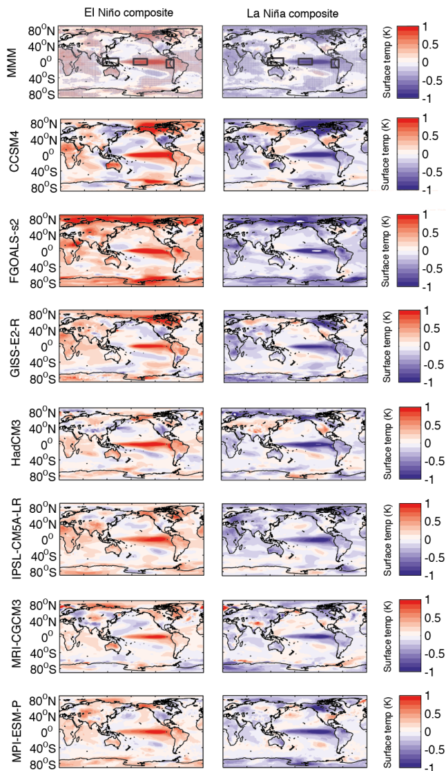
Figure 1. Composed anomaly maps for surface temperature (K) for CMIP5 models (left, El Niño episodes; right, La Niña episodes) for historical experiment, showing multi-model mean (MMM) and each model. Rectangular boxes indicate the West, Central and East Pacific regions. Stippling indicates where more than 80% of the models agree on the sign of the ENSO-associated anomaly.
