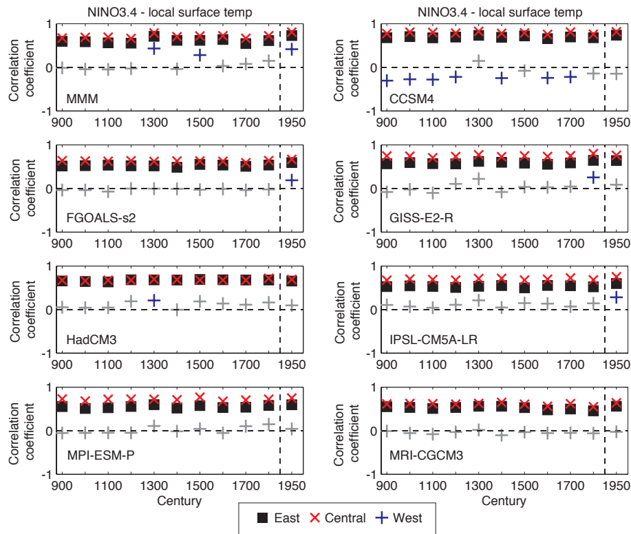
Figure 7. Area-mean correlation coefficients ( R ) of NINO3.4 and local surface air temperature for the East (black square), Central (red cross) and West (blue cross) calculated for the MMM, and for each model. Data points show correlation coefficients calculated for ten 100-year epochs comprising the Last Millennium simulation and for the historical simulation (1906–2005). Plot markers in grey indicate correlations that are not statistically significant (at the 5% significance level).
