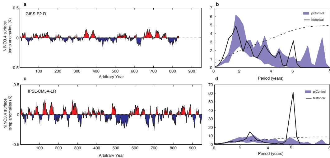
Figure 6. Running annual-mean surface temperature anomalies (K) over the NINO3.4 region ( 5^{\circ} N– 5^{\circ} S, 170^{\circ} – 120^{\circ} W) for extended piControl simulations conducted with GISS-E2-R (a) and IPSL-CM5A-LR (c) models. Red/blue shading highlights departures from each model's long-term mean. Running means were calculated using a 240-month triangle smoother. Control simulations are spun up to quasi-equilibrium and run for ideally >500 years, providing an arbitrary time series of model internal variability. Global mean NINO3.4 power spectrum ( K^2 /unit frequency, black), relative to the red-noise (AR(1)) benchmark (dashed) for GISS-E2-R (b) and IPSL-CM5A-LR (d) models.
