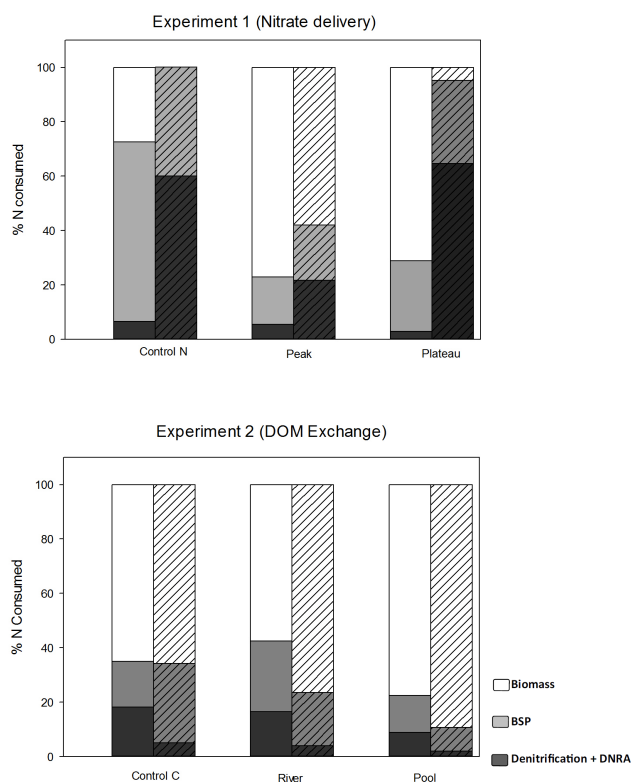
Fig. 5. Estimated percentage of total N pool used by denitrification and DNRA (dark gray), bacterial secondary production (middle gray) and biomass assimilation (light gray) using the five-day averages. Solid bars are estimates from the disconnected site, hashed bars from the restored site. N = 3 .
