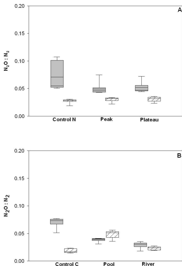
Fig. 4. Calculated \text{N}_2\text{O}:\text{N}_2 ratios over the five-day incubation from (A) Experiment 1: \text{NO}_3^- and (B) Experiment 2: DOM changes. Grey boxes are measurements from the disconnected site, hatched boxes from the restored site. Whiskers extend to the 95th and 5th percentiles. N = 33 .
