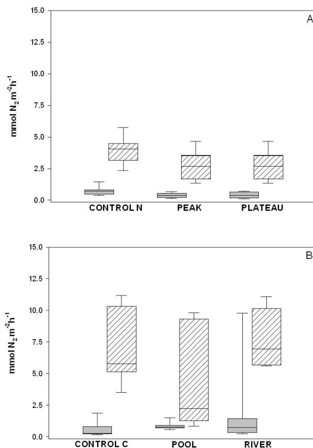
Fig. 3. Denitrification rates as measured over five days in (A) Experiment 1: \text{NO}_3^- and (B) Experiment 2: DOM changes. Grey boxes are measurements from the disconnected site, hatched boxes from the restored site. Whiskers extend to the 95th and 5th percentiles. N = 33 .
