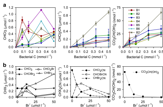
Fig. 1. Formation of some C1/C2 organohalogenes by halogenation of bacteria. (a) effects of bacterial C concentrations (at 0.0, 0.083, 0.167, 0.333, and 0.50 \text{ mmol l}^{-1} ). Error bars show SD from 3 replicates. (b) effects of bromide (at 0, 6.25, 12.5, 25, and 50 \mu\text{mol l}^{-1} from KBr) taking Staphylococcus sciuri at 0.5 \text{ mmol-C l}^{-1} as example. B1: Acinetobacter junii ; B2: Aeromonas hydrophila ; B3: Bacillus cereus ; B4: Bacillus subtilis ; B5: Escherichia coli ; B6: Shigella sonnei ; and B7: Staphylococcus sciuri .
