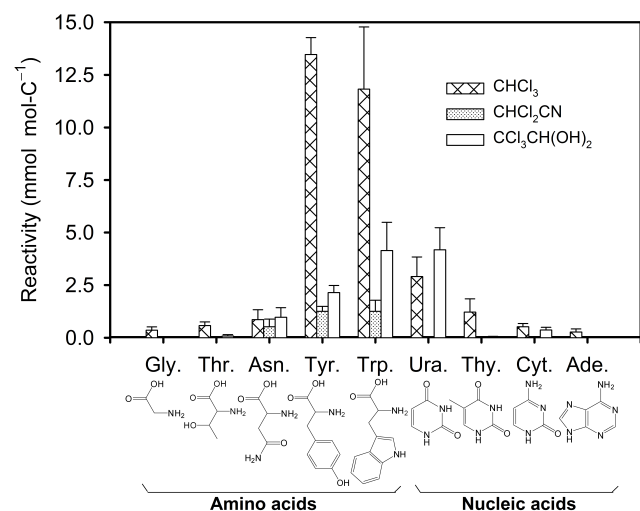
Fig. 2. Halogenation reactivity of 9 bacterial cellular monomers. Error bars show standard deviation from a total of 10 replicates (two for each C concentration: 0.083, 0.167, 0.250, 0.333, and 0.5 mmol C l -1 ).
