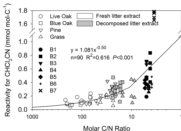
Fig. 3. Reactivity of dichloro-acetonitrile formation for extracts of fresh litter ( n = 32 ), decomposed litter ( n = 30 ) and bacterial suspensions ( n = 28 ) along a C/N ratio gradient. B1–B7 refer to the same seven different bacterial strains in Fig. 1.
