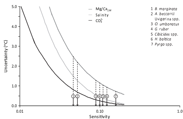
Fig. 4. Temperature uncertainty caused by variability in salinity (1), Mg/Ca SW ( 0.6 \text{ mol mol}^{-1} ) and carbonate ion concentration ( 50 \mu\text{mol kg}^{-1} ). Temperature uncertainties are calculated at 8 °C using the Mg/Ca–temperature calibration for B. marginata with a changing temperature sensitivity (exponential constant). Temperature sensitivities used for the different species are from Table 4. Mg/Ca parameter relations from a number of studies were used to calculate the uncertainty in temperature. Mg/Ca SW : Wit et al. (2012). Salinity: Dueñas-Bohórquez et al. (2009). Carbonate ion concentration: Dueñas-Bohórquez et al. (2011b).
