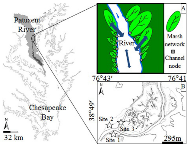
Fig. 1. Study area located in the tidal freshwater portion of the upper Patuxent River, Maryland. (A) Schematic diagram showing the organization of tidal marshes along the river. Tidal fluxes are controlled by inlet channel geomorphology (governing node). (B) Map of selected marshes for mass balance measurements. Marsh areas ( m^2 ) are as follows: Site 1: 670.6, Site 2: 5705, Site 3: 536 873.4.
