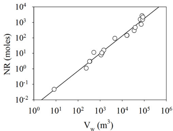
Fig. 7. Relationship between net nitrate retention over a tidal cycle and water volume. Data are reported for the three sampling sites for various tides in 2008, 2010, and 2011. Nitrate retention is a simple function of hydrologic flux that varies over 5 orders of magnitude. Seasonal multi-year data for spring (high tides) follow the relationship: NR = 0.0045V_w^{1.1} ( n = 13 , R^2 = 0.98 ).
