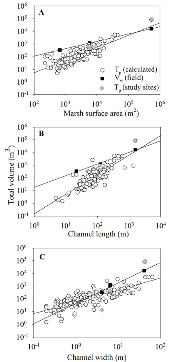
Fig. 6. Relationship of calculated tidal prism to (A) marsh surface area, (B) channel length, and (C) inlet channel width. Field measurements are shown as black squares; gray diamonds highlight predicted tidal prism for the corresponding study sites.
