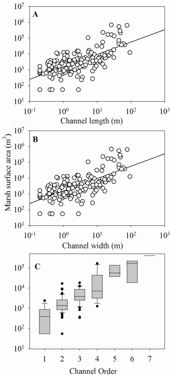
Fig. 4. Geomorphic relationships of channel order, inlet width, and total channel length to marsh surface area of tidal freshwater marshes along the Patuxent River estuary. (A) L = 1.3A^{0.53} ( n = 142 , R^2 = 0.79 ). (B) W = 0.2A^{0.65} ( n = 142 , R^2 = 0.47 ). Standard error is less than the size of each data point. (C) Box plot of marsh surface areas for each stream order.
