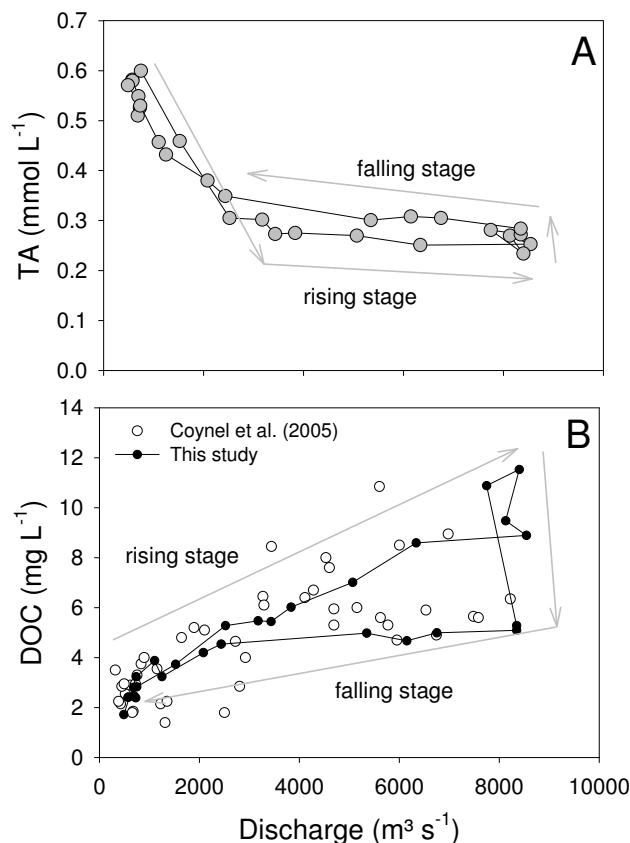
Fig. 9. Seasonal variations of (A) total alkalinity, and (B) dissolved organic carbon concentrations, showing different hysteresis patterns. DOC data from this study are compared with data from Coyne et al. (2005).
