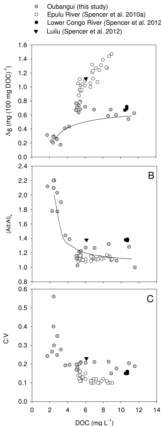
Fig. 11. Covariation between dissolved organic carbon concentrations and (A) carbon-normalized lignin yields ( \Lambda_8 ), (B) (\text{Ad:Al})_v ratios, and (C) C:V ratios, for the Oubangui River at Bangui between March 2010 and March 2011 (grey symbols), along with literature data from other locations in the Congo River basin (open and black symbols, see legend). Lines on (A) and (B) show a theoretical two end-member mixing scenario (see text for details).
