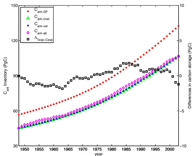
Fig. 4. Changes in the estimated ocean C_{\text{ant}} inventories, estimated using the GF method and the CCSM, through time (the left axis) and the differences in total DIC inventory from two simulations forced with rising atmospheric CO 2 (the right axis). Shown are: C_{\text{ant\_GF}} (red crosses); C_{\text{ant\_cnst}} (green triangles); C_{\text{ant\_var}} (blue crosses); C_{\text{ant\_all}} (magenta diamonds). The black squares show the differences between total DIC in the Texp and in the Cexp. \Delta_{\text{Texp-Cexp}} = C_{\text{ant\_all}} - C_{\text{ant\_cnst}} .
