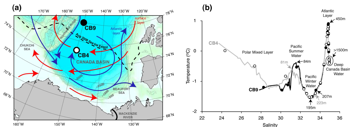
Fig. 1. (a) Sampling stations CB4 and CB9 in the Canada Basin are mapped along with surface (red) and Atlantic (blue) water layer currents (McLaughlin et al., 2009; Stein and Macdonald, 2004) and the approximate sea-ice extent in August 2008 ( http://nsidc.org/data/ ). (b) Water masses in the Canada Basin are characterized by temperature and salinity. Solid lines (grey-CB4; black-CB9) show real-time measurements from sensors attached to the rosette. Discrete points correspond to bottle samples collected for isotopic analyses of DIC and DOC. Displayed depths are used to translate labeled water masses onto depth profiles (Fig. 2).
