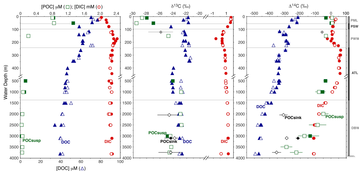
Fig. 2. Full-depth carbon isotope profiles of DOC (blue triangles), POCsusp (green squares), and DIC (red circles) at sites CB4 (open symbols) and CB9 (filled symbols) in the Canada Basin in August 2008. POCsink (black diamonds) represents a flux-weighted average from time-series sediment traps at water depths of 2050 m (2008–2009), 3100 m (2004–2005; 2007–2009), and 3750 m (2008–2009) (Hwang et al., 2012). POCsink at 120 m (grey diamonds) is derived from an ice-tethered sediment trap that traversed the Canada Basin and Chukchi Rise in 1997–1998 (Honjo et al., 2010). POCsink error bars show \pm 1 SD for each corresponding time series. Error bars for POCsusp reflect propagated errors ( \pm 1 SD) from procedural blank and DOC corrections; DOC errors ( \pm 1 SD) reflect propagated errors of blank corrections. Error bars ( \pm 1 SD) for DIC reflect analytical uncertainty only. When not visible, error bars are smaller than symbols. Water masses (Polar Mixed Layer – PML; Pacific Summer Water – PSW; Pacific Winter Water – PWW; Atlantic Layer – ATL; and Deep Canada Basin Water – DBW) are delineated according to characteristic temperature and salinity (see Fig. 1b). These data are available in the Supplement in Tables S1–S3.
