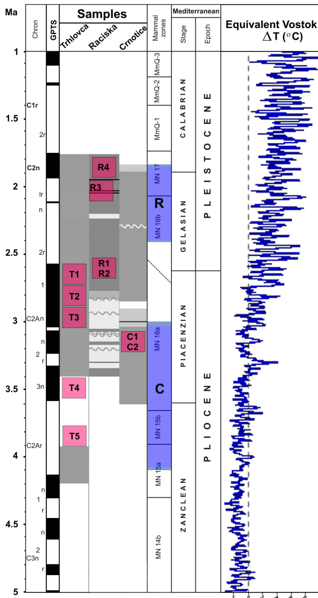
Fig. 4. A correlation of the obtained magnetostratigraphic results with the standard paleomagnetic scale (GPTS; after Cande and Kent, 1995; modified after Horáček et al., 2007), mammal zones, temperature estimates (after Lisiecki and Raymo, 2005) and position of the samples with invertebrates (in red) and vertebrates (in blue): T = Trhlovca Cave, R = Račiška Cave, C = fossil cave in the Črnotiče Quarry.
