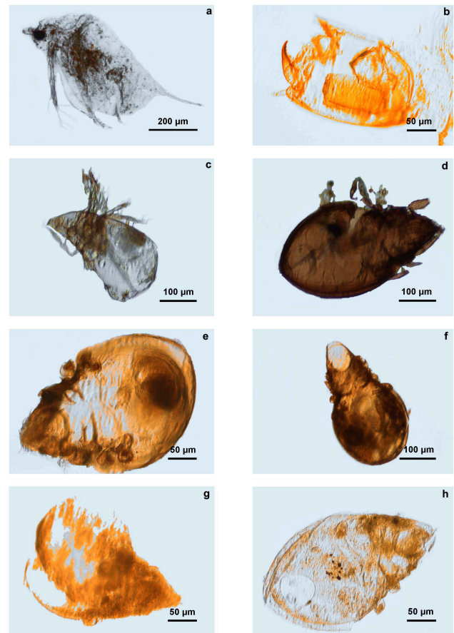
Fig. 3. Light microscope photographs of the identified fossil invertebrates in the cave sediments in Slovenia: (a) Daphnia sp.; (b) Orthocladinae; (c) Dissorhina n. sp.; (d) Zygoribatula frisiatae ; (e) Miracarus n. sp.; (f) Opiella (cf. Rhinoppia ) n. sp. 1; (g) Suctobelbella sp. ?; (h) Opiella ( Rhinoppia ) n. sp. 2.
