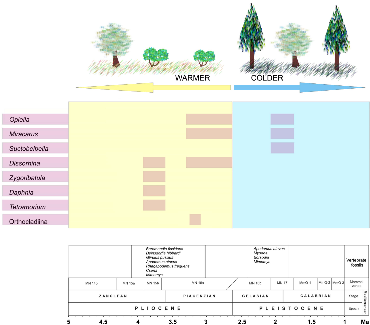
Fig. 5. Invertebrate fossils found in the studied caves, correlated with climate, vegetation and fossil vertebrates.
