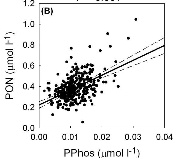
Fig. 7. Bivariate plots of (A) particulate organic carbon POC vs. PPhos and (B) PON vs. PPhos for euphotic zone (0–100 m) particles during this study period. The solid line in each panel is the least squares linear regression and dashed lines are the 95% confidence interval. Regression equations ( \pm stdev) are given above each panel.
