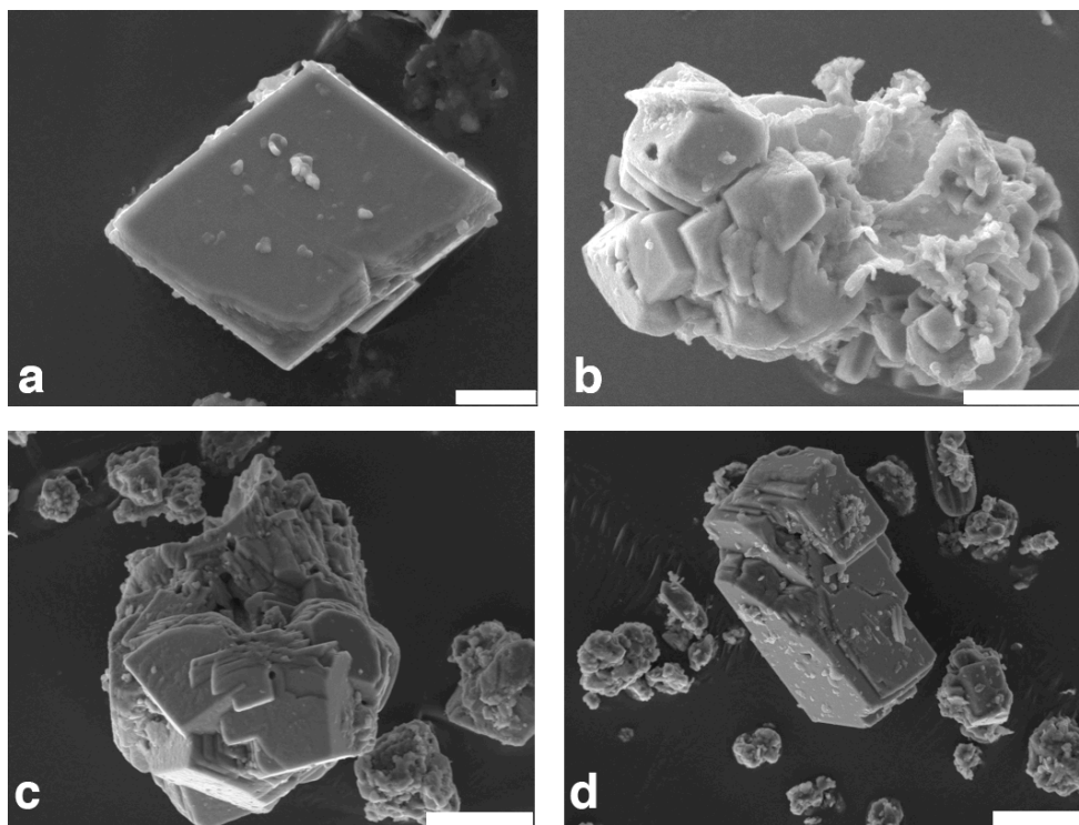
Fig. 5. SEM images from carbonate crystals: (a) authigenic calcite crystals from sediment trap 2d (mooring 2, at 6.5 m depth; bar length = 5 µm); (b) large idiomorphic calcite crystal clusters from trap 1b (mooring 1, at 5.6 m depth). Note the hole from cyanobacteria-mediated crystallization (bar length = 10 µm); (c) large idiomorphic calcite crystal cluster from core 08 at 15 cm depth, recovered ~100 m away from the spring zone (bar length = 20 µm). Note similar holes as in b); (d) large idiomorphic calcite crystal clusters from core 05 at 15 cm depth recovered in the spring zone (bar length = 20 µm).
