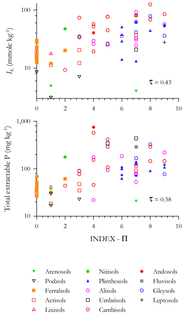
Fig. 15. Trade off between soil element concentrations and limiting physical properties. Effective cation exchange capacity ( I_E , top) and total extractable phosphorus (below) co-vary with soil physical limitations. Values of Kendall's \tau rank correlation coefficient are also shown.
