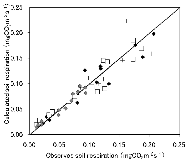
Fig. 5. Comparison of observed and calculated respiration rate in Kahoku Experimental Forest. Cross: Plot T. Black diamond: Plot U. White square: Plot M. Gray diamond: Plot L.
