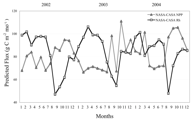
Fig. 3. Monthly patterns of the NASA-CASA predicted NPP and R_h fluxes at the Tapajós National Forest (TNF) tower flux site.
