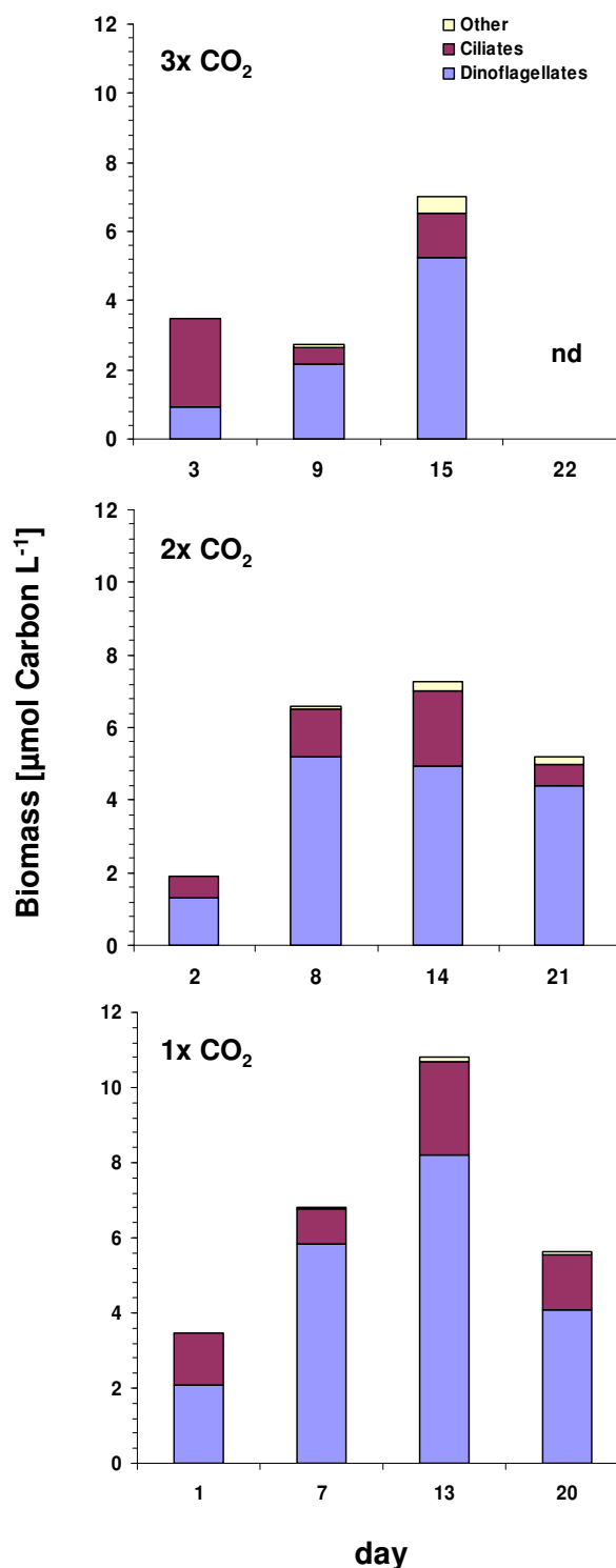
Fig. 1. Relative biomasses (μmol C l -1 ) of major groups of heterotrophic protists at start ( t 0 ) of the respective experiments in the ambient mesocosm water. Data are shown for CO 2 -treatments 1×, 2×, 3× at the respective day of experiment (1–22). Data from 3× CO 2 on day 22 are missing (=not determined, nd).
