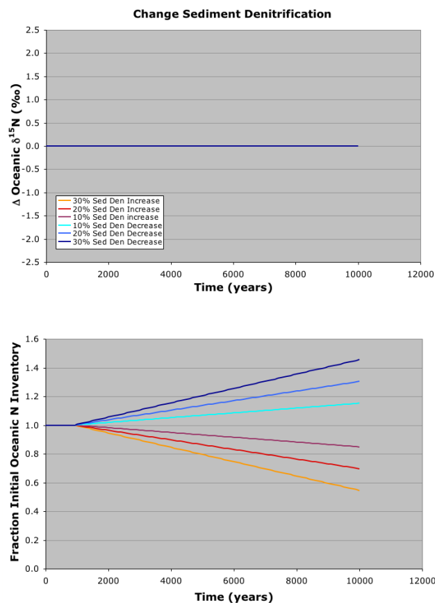
Fig. 5. Temporal evolution of oceanic \delta^{15}\text{N} (top) and N inventory (bottom) with up to \pm 30\% changes in sedimentary denitrification. Initial conditions are of steady state and 50% contributions from water column and sedimentary denitrification respectively. The value for \epsilon_{\text{den}} (effective) for water column denitrification is 12‰. Because sedimentary denitrification is considered non-fractionating, no change in \delta^{15}\text{N} occurs despite changes in N inventory.
