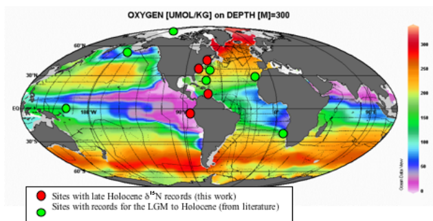
Fig. 6. Location map for sediment \delta^{15}\text{N} records discussed in this paper. High-resolution, good fidelity records spanning the late Holocene are distinguished from those that cover the last glacial maximum but have poor temporal resolution and likely diagenetic influence. Oxygen at 300 m is contoured for reference to show locations of subsurface suboxic zones which sustain water column denitrification (data from the eWOCE database).
