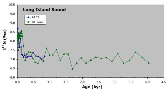
Fig. 7. Long Island Sound sediment \delta^{15}\text{N} records spanning the last 4 kyr. Age model established from ^{14}\text{C} dating, and known pollen and contaminant horizons. The increase in \delta^{15}\text{N} within the last 200 years corresponds to the onset of anthropogenic eutrophication.
