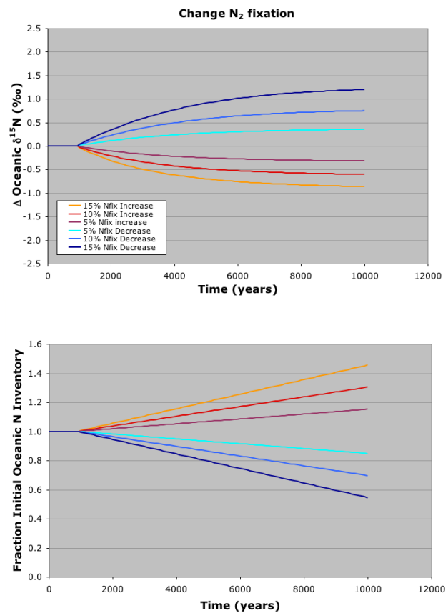
Fig. 3. Temporal evolution of oceanic \delta^{15}\text{N} (top) and N inventory (bottom) with up to \pm 15\% changes in total \text{N}_2 fixation (assumed to be sole source). Initial conditions are of steady state and 50% contributions from water column and sedimentary denitrification respectively. The value for \epsilon_{\text{den.}} (effective) is 12%. Sedimentary denitrification is considered non-fractionating.
