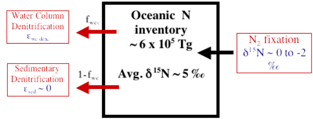
Fig. 1. Schematic of the simple box model used to explore the influence on average oceanic \delta^{15}\text{N} and the relative proportions of N sources and sinks as well as variations in the effective N isotopic fractionation ( \epsilon_{\text{den.}} ) associated with water column denitrification. The model is used under both steady and non-steady conditions. Accepted values for isotopic composition, fractionation effect, N inventory, and N fluxes are shown for reference.
