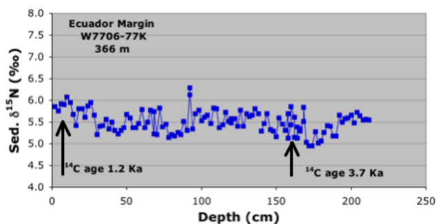
Fig. 10. Sediment \delta^{15}\text{N} record from a site on the Ecuadorian continental margin. Due to the few ^{14}\text{C} dates, the x-axis is depth in core and the dates are noted on the figure.
