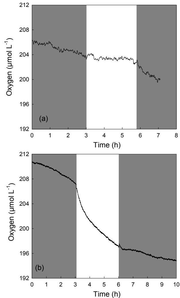
Fig. 3. Oxygen time course during incubation of water from Southwest lagoon of New Caledonia. Shaded boxes represent the dark periods and unshaded box represents the illumination period. Samples were collected in N12 on 16 March 2005 (a) and in M41 on 11 May 2006 (b), concentration of chlorophyll a was 0.75 \mu\text{g L}^{-1} (a) and 0.27 \mu\text{g L}^{-1} (b). See Table 1 for rate values.
