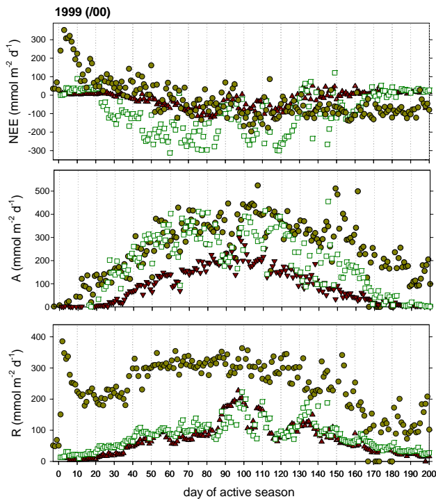
Fig. 1. Daily net ecosystem-atmosphere exchange of CO 2 (NEE), and component fluxes ecosystem assimilation ( A ) and respiration ( R ) in ecosystems representing the semi-arid tropics (Mopane woodland, Botswana) and the cold-continental boreal biome (Scots pine forest and mire, Siberia). Data are from eddy covariance measurements conducted during the active period 1999/2000 (Botswana) and 1999 (Siberia), denoted as Mopane: dark yellow circles, Mire: dark red triangles, and Pine: green open squares. The derivation of ecosystem assimilation and respiration from NEE measurements is described in the text. Following meteorological standards NEE are denoted as negative when directed into the system ( A > R ). However, in the manuscript the fluxes are analysed with respect to basic ecophysiological theory and assimilation as well as respiration are plotted as positive values.
