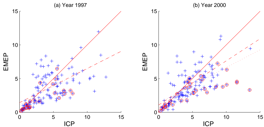
Fig. 13. Wet Deposition of \text{NH}_4^+ -N in open field, \text{kg(N) ha}^{-1} \text{yr}^{-1} . EMEP modelled wet vs. ICP bulk precipitation during 1997 and 2000. Lines and symbols as per Fig. 3.
