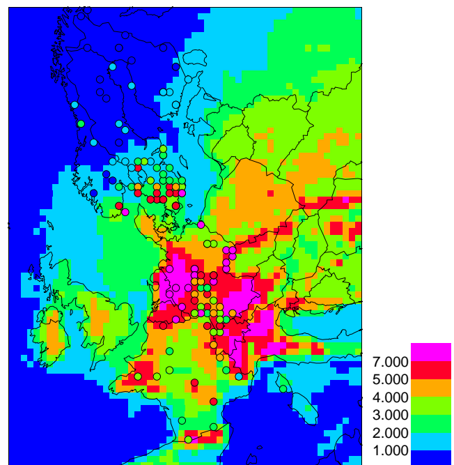
Fig. 15. Yearly average wet deposition of reduced nitrogen, \text{kg(N) ha}^{-1} \text{yr}^{-1} . EMEP modelled wet deposition (deposition field) vs. ICP (bullets) during 1997.
