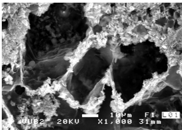
Fig. 2. Continued. (g) Bridging and inter-space filling, fungal biomineralization bridging original attacked dolomite grains. The mineral-bridge is composed of Ca-oxalates. The empty space between the grains is filled with newly produced minerals (Ca-oxalates). (h) Honey-comb structure formed by preferential deposition of biominerals (Ca-oxalates) on original grain boundaries and void creation by fungal attack and dissolution of those grains. The image also shows the depth of the dissolution. Bar scale: a=100 \mu\text{m} ; b, c, d, e, g, h=10 \mu\text{m} ; f=1 \mu\text{m} .
