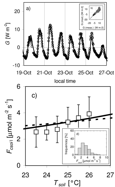
Fig. 10. (a–b) Predicted (open circles) and measured (solid line) in (a) soil heat flux ( G ) at the tower RBJ-A in 1999 using a constant bulk ( 0-1 \text{ m} ) soil surface conductance for heat ( 1/g_{soil}H=500 \text{ s m}^{-1} ). The linear fit shown in (b) predicts y=1.02x + 0.92 ( r^2=0.92 ). (c–d) Parameterization of soil respiration ( F_{csoil} ) using continuous measurements from three soil chambers and soil temperature ( T_{soil} ) measured at -0.05 \text{ m} in 1999 (dry season data from the Jaru site, RBJ-A tower, see Table 2). (c) Mean observations and standard deviations for 0.5^{\circ}\text{C} intervals (open squares) and predictions of Eq. (30) using an optimal Q_{10} \approx 1.6 (dashed line) and Q_{10} \approx 2.3 (solid line) as derived by Meir et al. (1996) for another site. (d) Frequency distribution of F_{csoil} (total N=269 ).
