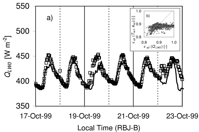
Fig. 5. Observed and predicted Atmospheric emissivity ( \epsilon_{a0} ) and incoming long-wave radiation ( Q_{LW0} ) at the tower RBJ-B for one week period. (a) Measured (open squares) and predicted time series (solid line) for Q_{LW0} . (b) \epsilon_{a0}(T_{ref}, e_{ref}) plotted against \epsilon_{a0}(Q_{LW0}) (parameterized versus observed atmospheric emissivity, respectively).
