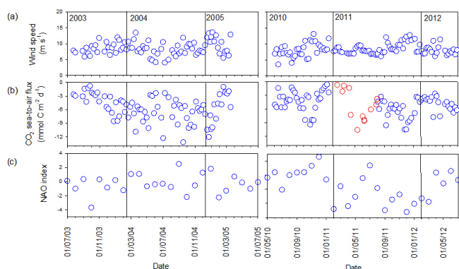
Figure 5. Data from 2003 to 2005 and 2010 to 2012 (blue circles) for (a) weekly satellite wind data in the region of the PAP-SO; (b) calculations of weekly sea-to-air CO 2 flux (negative: into the ocean) from in situ PAP-SO p(\text{CO}_2) data and satellite wind (see text for details) with additional flux calculations from SOO data (red circles); (c) the monthly NAO index.
