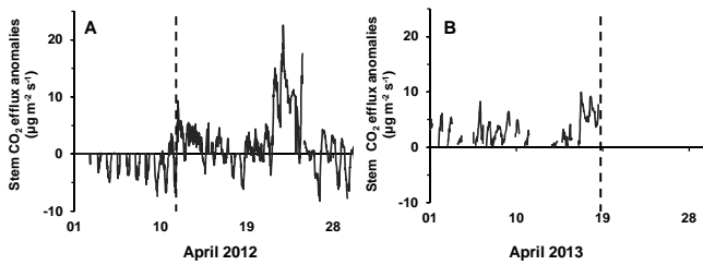
Figure 8. Temperature-corrected stem CO 2 efflux anomalies for April 2012 (a) and 2013 (b).
