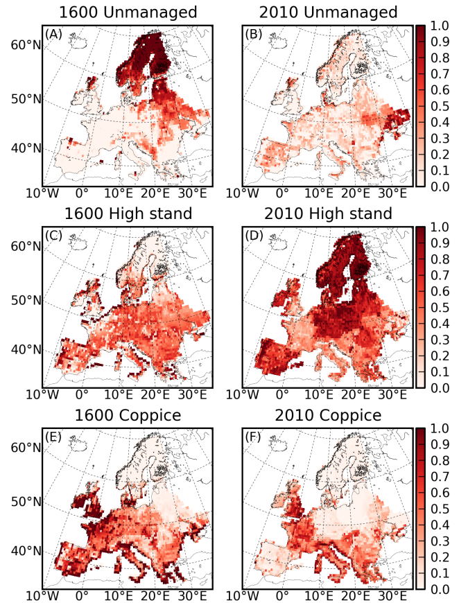
Figure 6. Distribution of management strategies over Europe. (a) Unmanaged forests in 1600 and (b) in 2010. (c) High-stand forests in 1600 and (d) in 2010. (e) Coppice management in 1600 and (f) in 2010. The color bar shows the fraction of the forest managed by a given strategy. Pixels along the coastlines often contain few forests, frequently resulting in the entire pixel being under a single management strategy.
